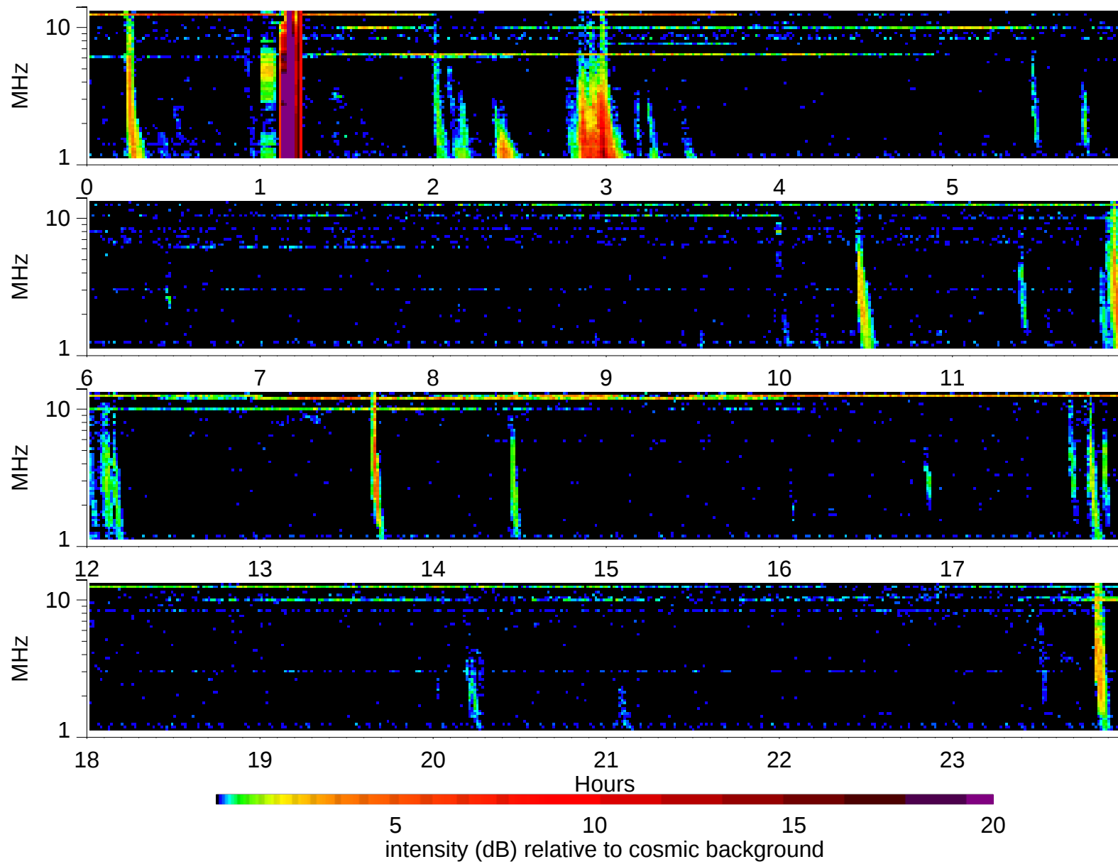
Wind Waves RAD2 receiver: 2002/5/12
