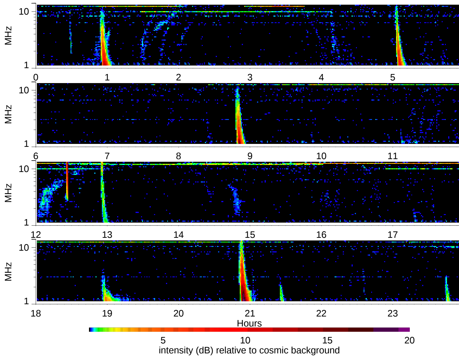
Wind Waves RAD2 receiver: 2002/5/13
