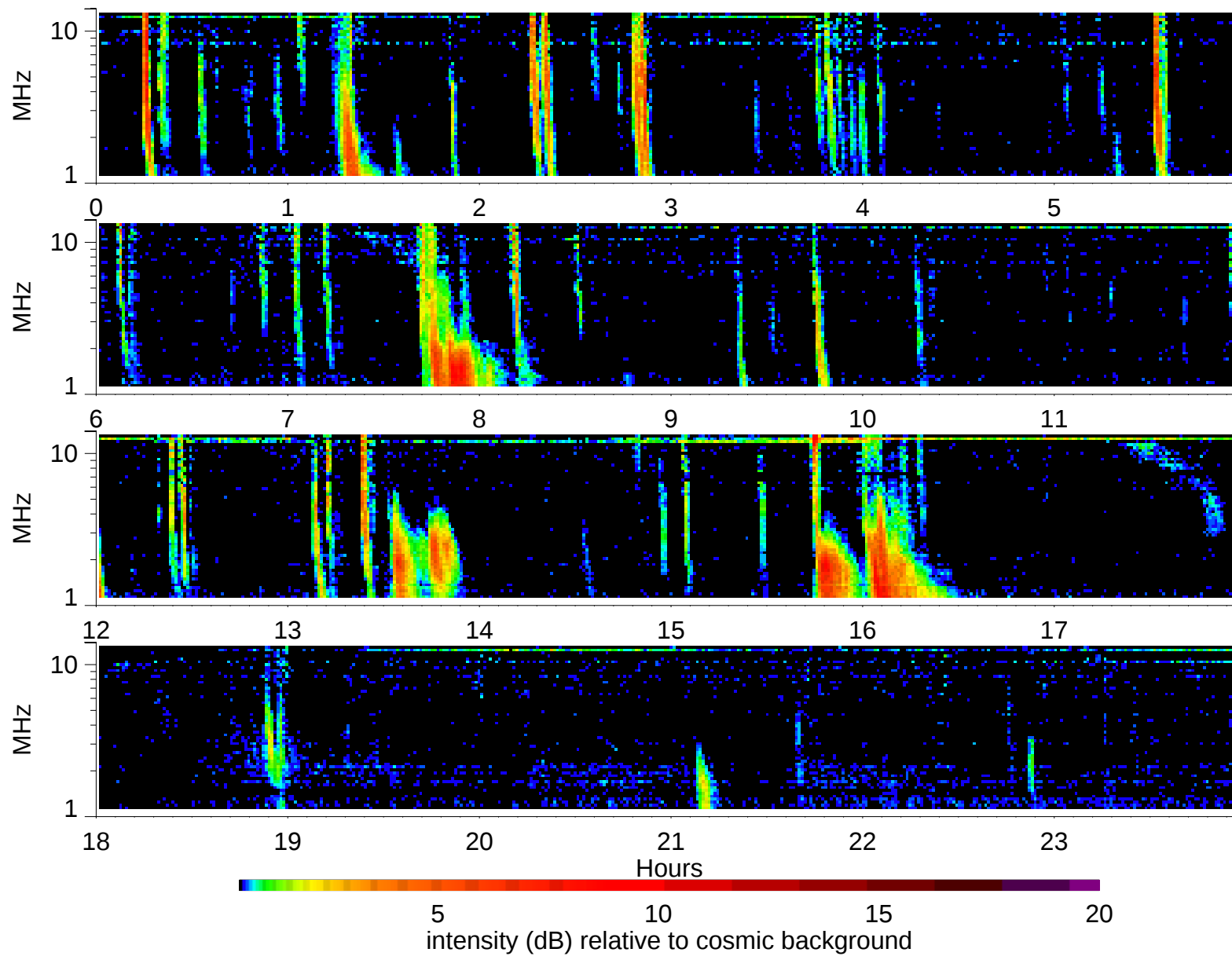
Wind Waves RAD2 receiver: 2002/5/17
