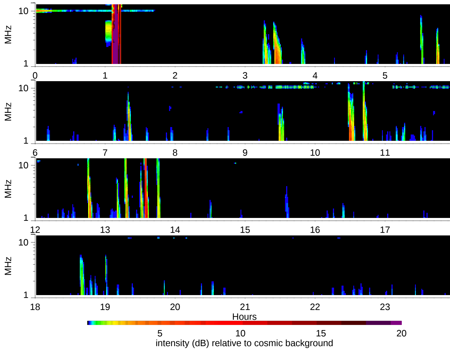
Wind Waves RAD2 receiver: 2002/5/24
