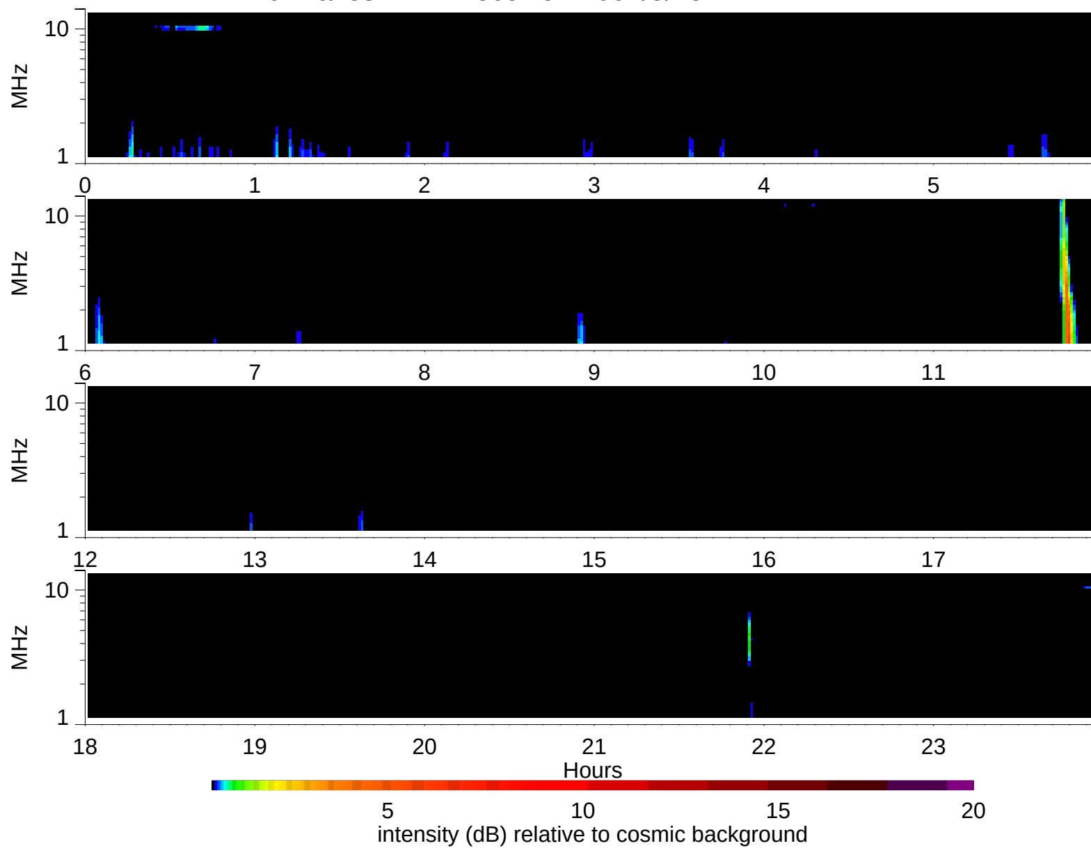
Wind Waves RAD2 receiver: 2002/5/25
