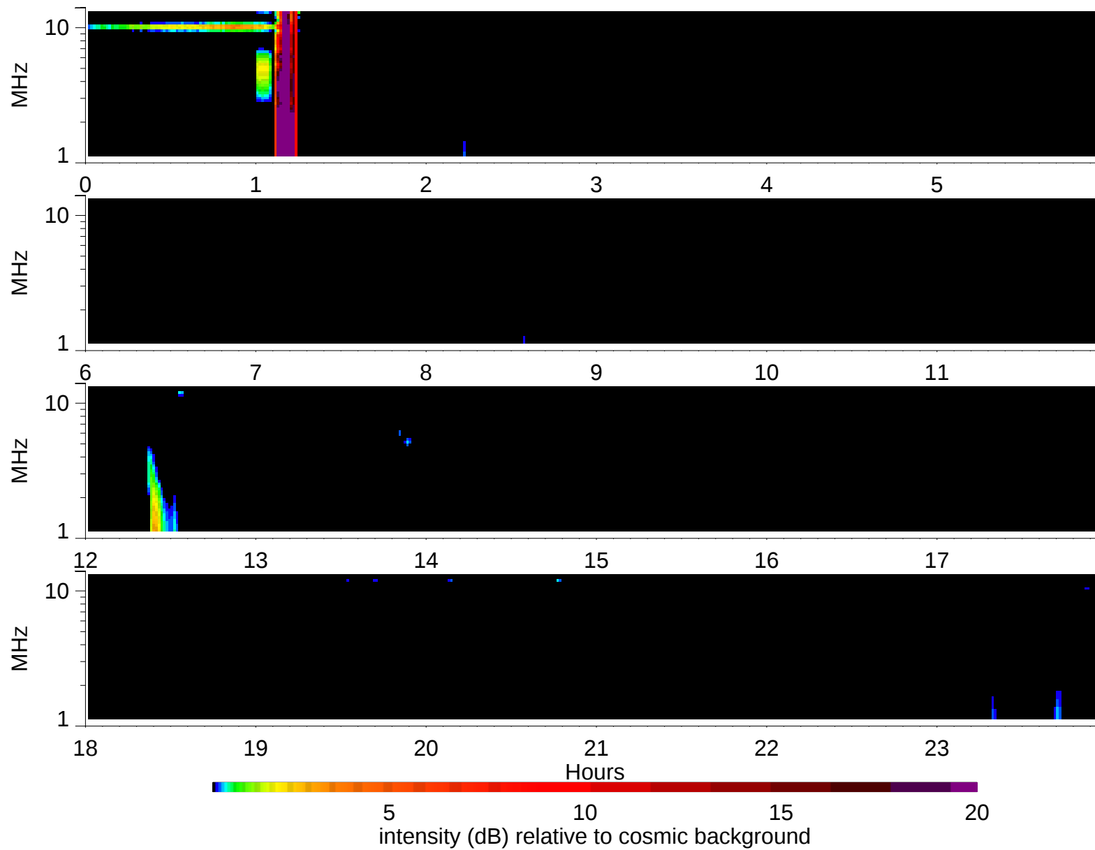
Wind Waves RAD2 receiver: 2002/5/26
