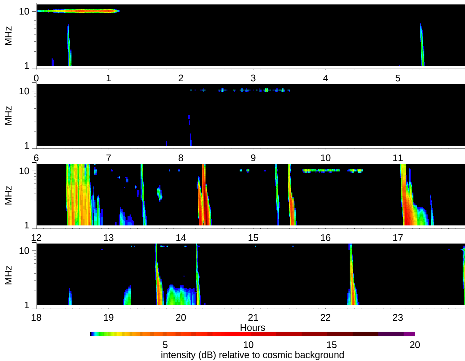
Wind Waves RAD2 receiver: 2002/5/27
