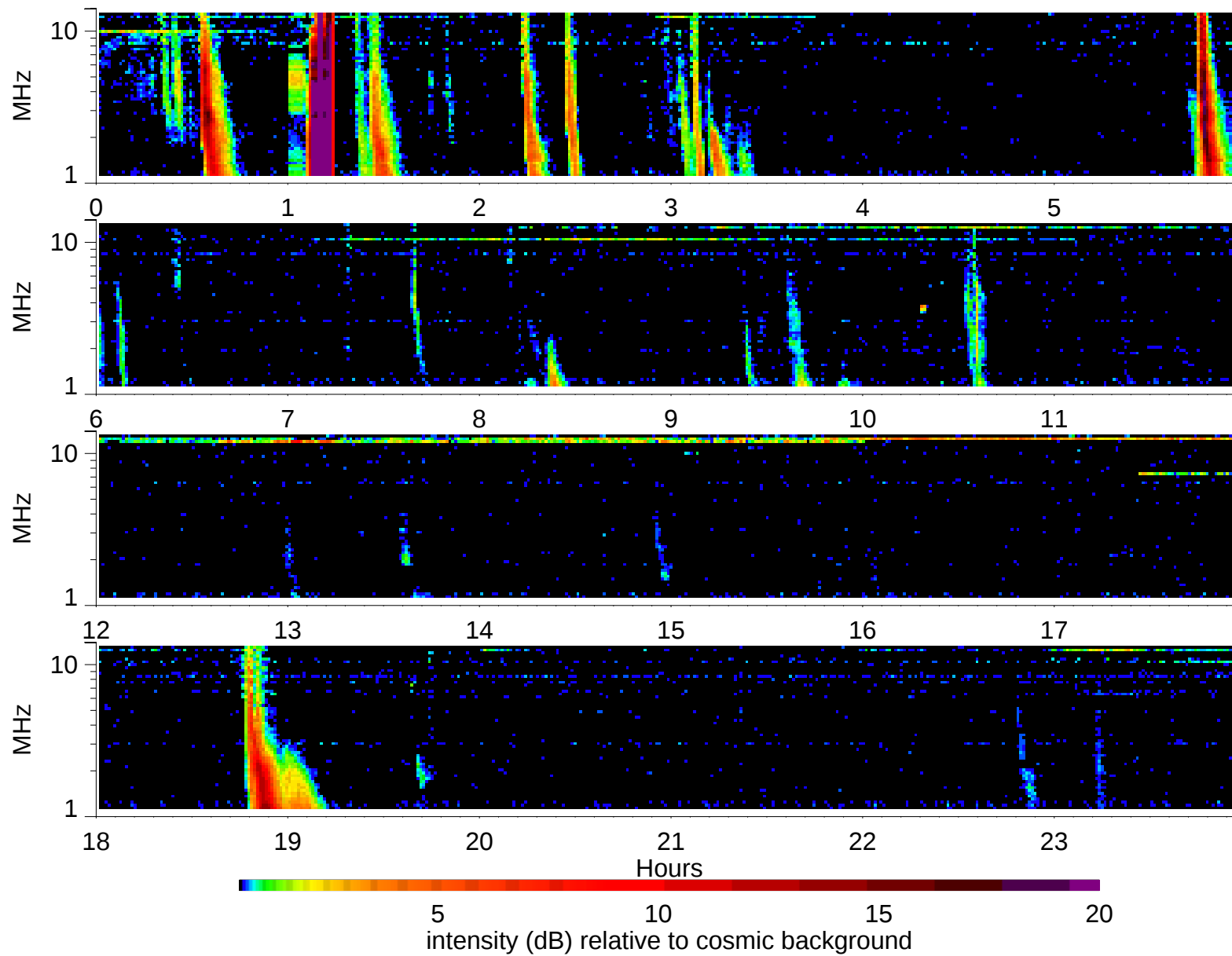
Wind Waves RAD2 receiver: 2002/6/5
