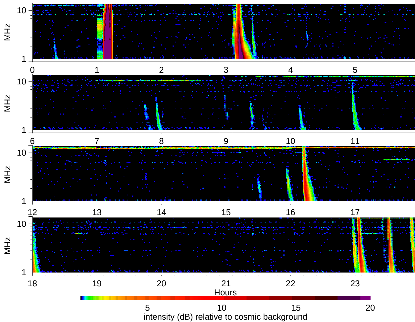
Wind Waves RAD2 receiver: 2002/6/7
