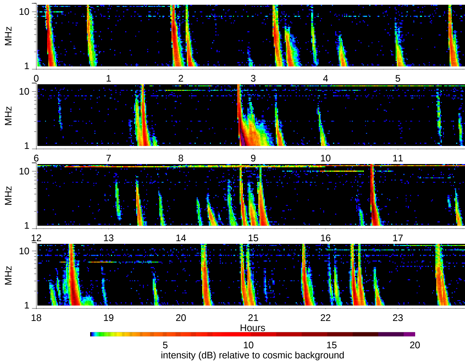
Wind Waves RAD2 receiver: 2002/6/8
