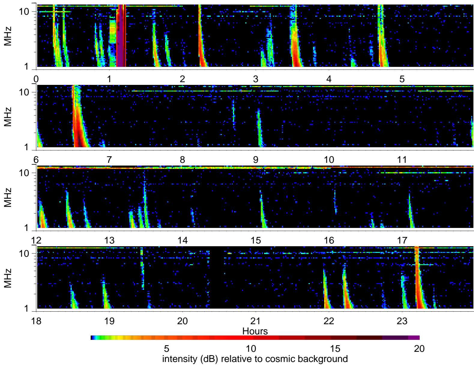
Wind Waves RAD2 receiver: 2002/6/9
