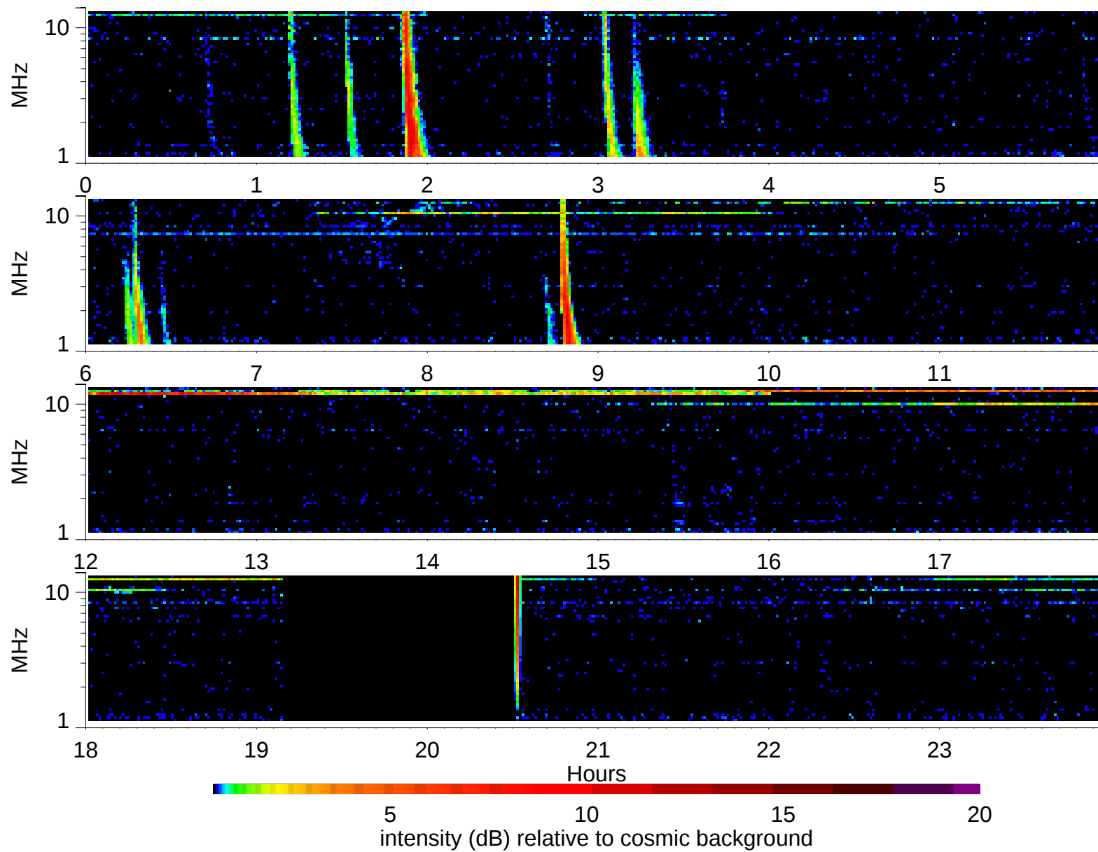
Wind Waves RAD2 receiver: 2002/6/10
