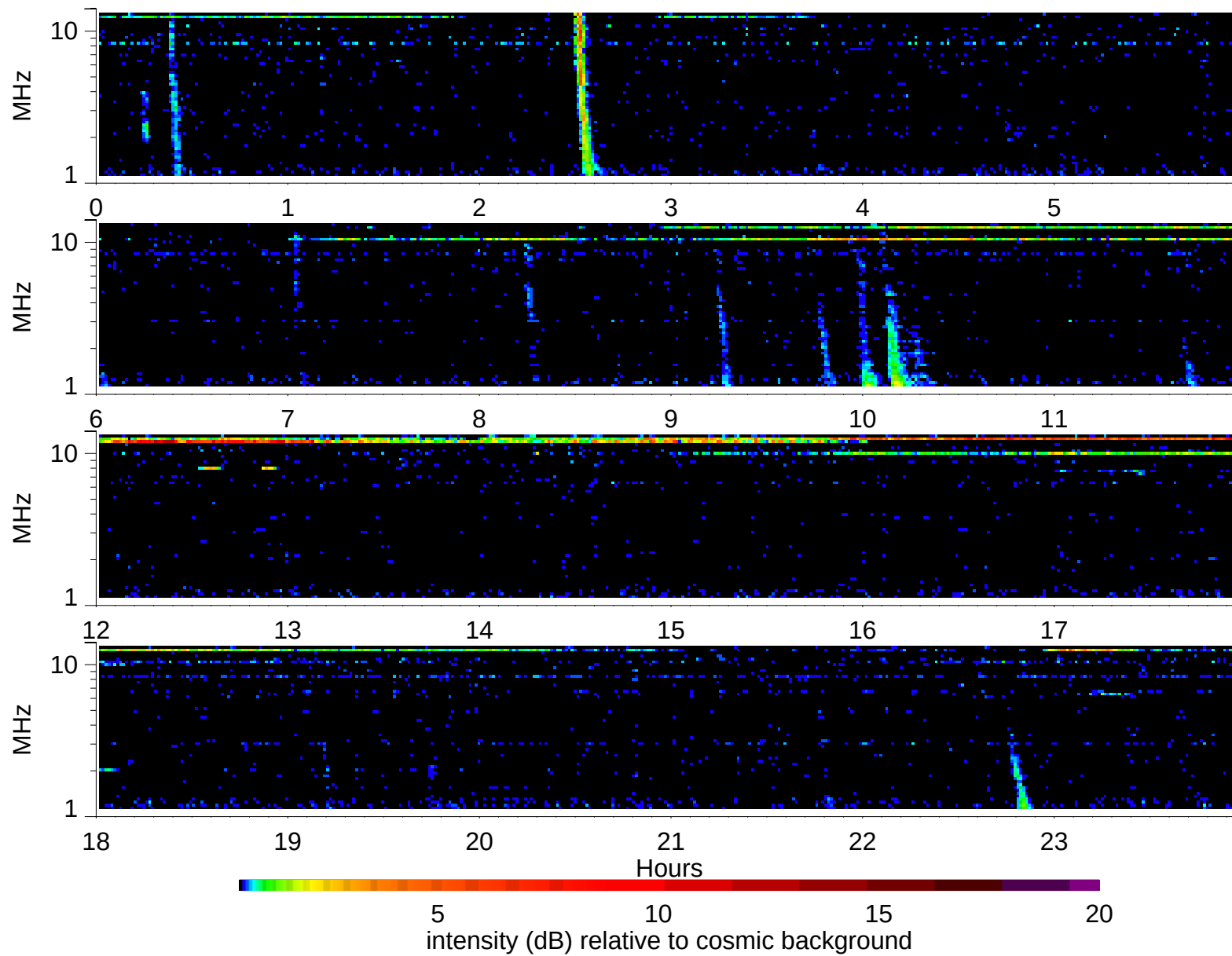
Wind Waves RAD2 receiver: 2002/6/14
