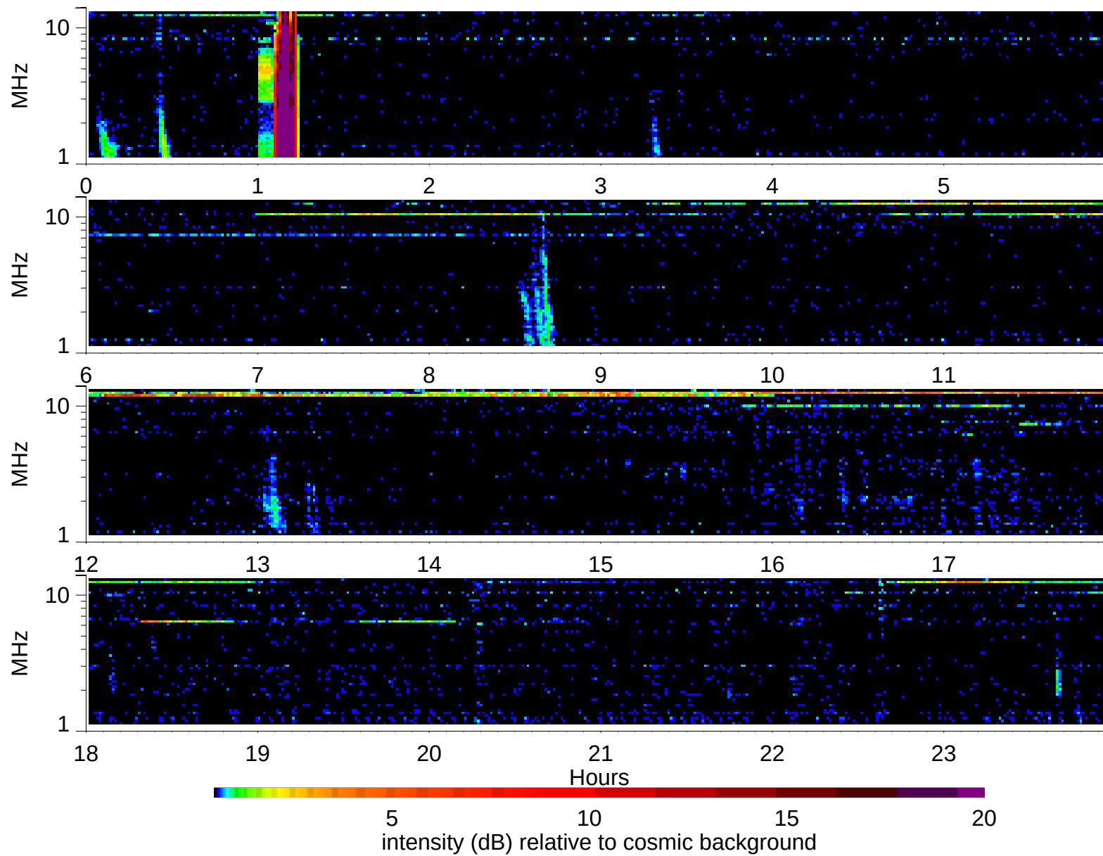
Wind Waves RAD2 receiver: 2002/6/15
