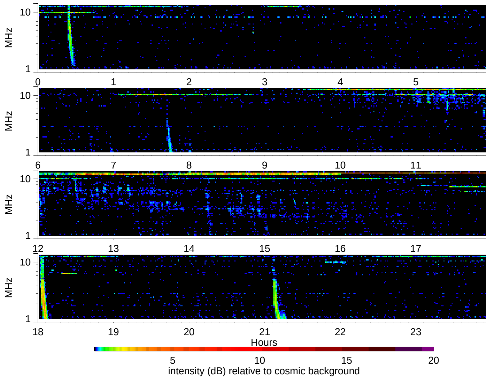
Wind Waves RAD2 receiver: 2002/6/16
