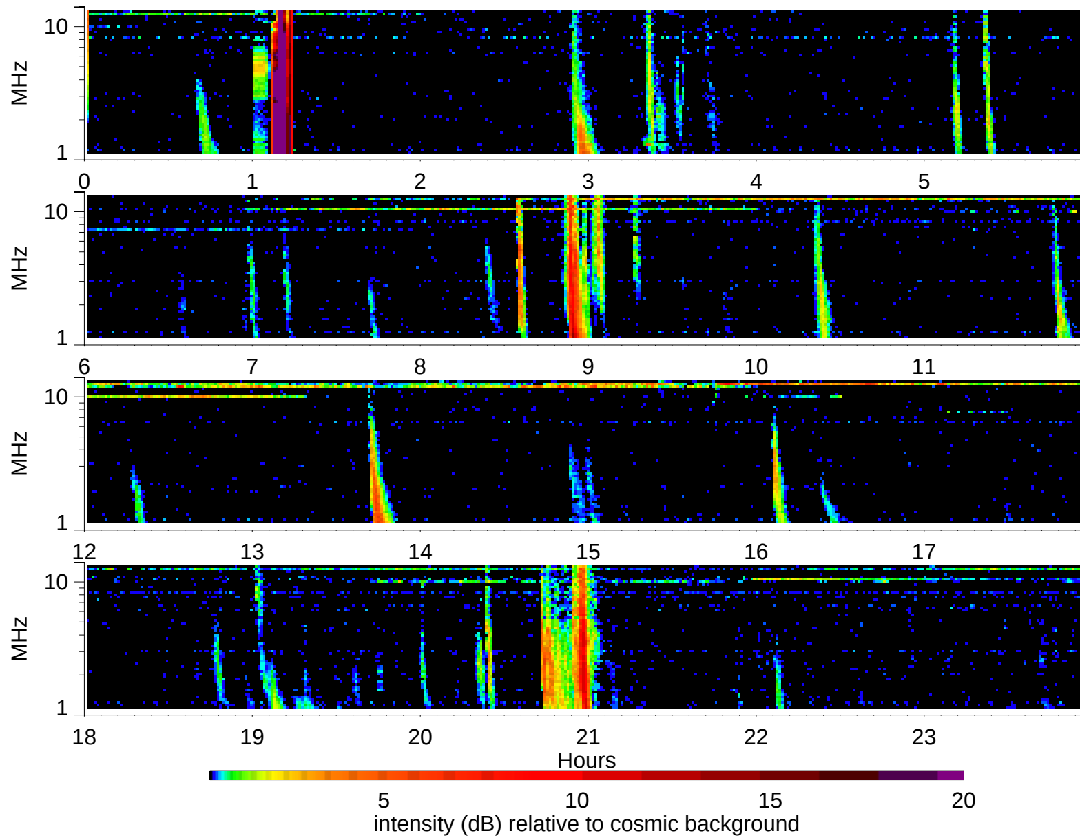
Wind Waves RAD2 receiver: 2002/6/19
