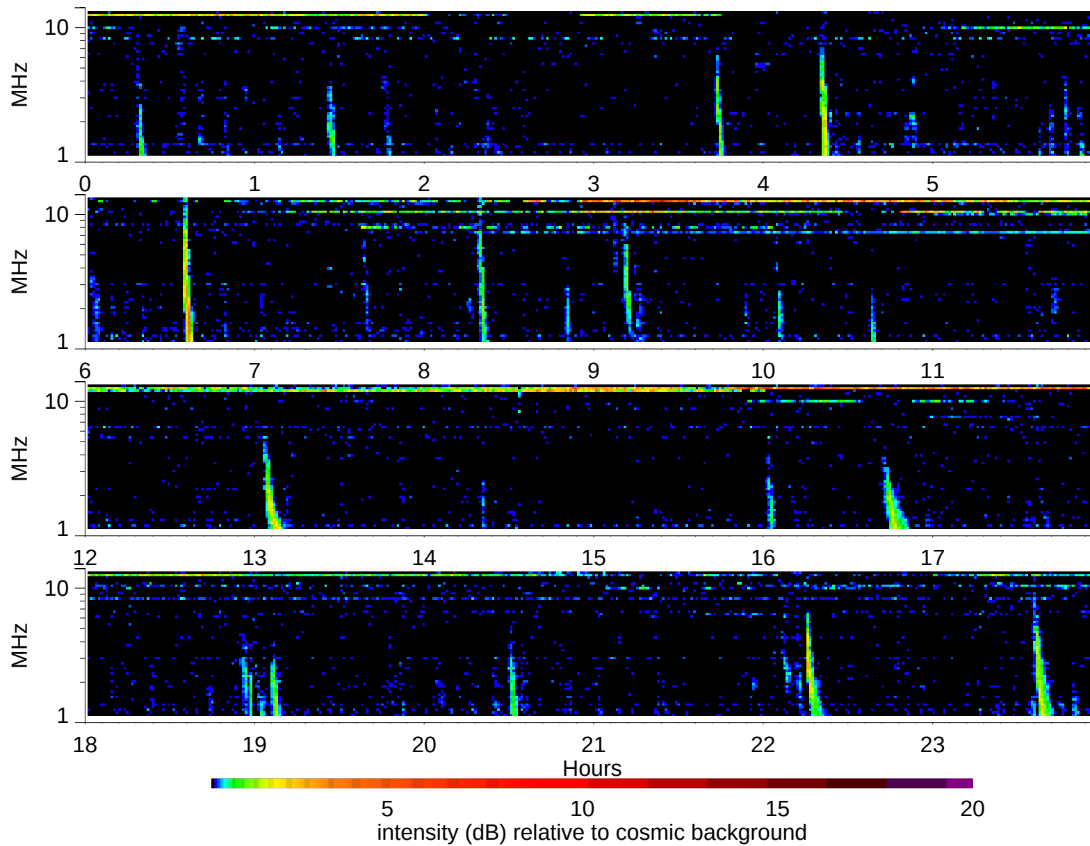
Wind Waves RAD2 receiver: 2002/6/20
