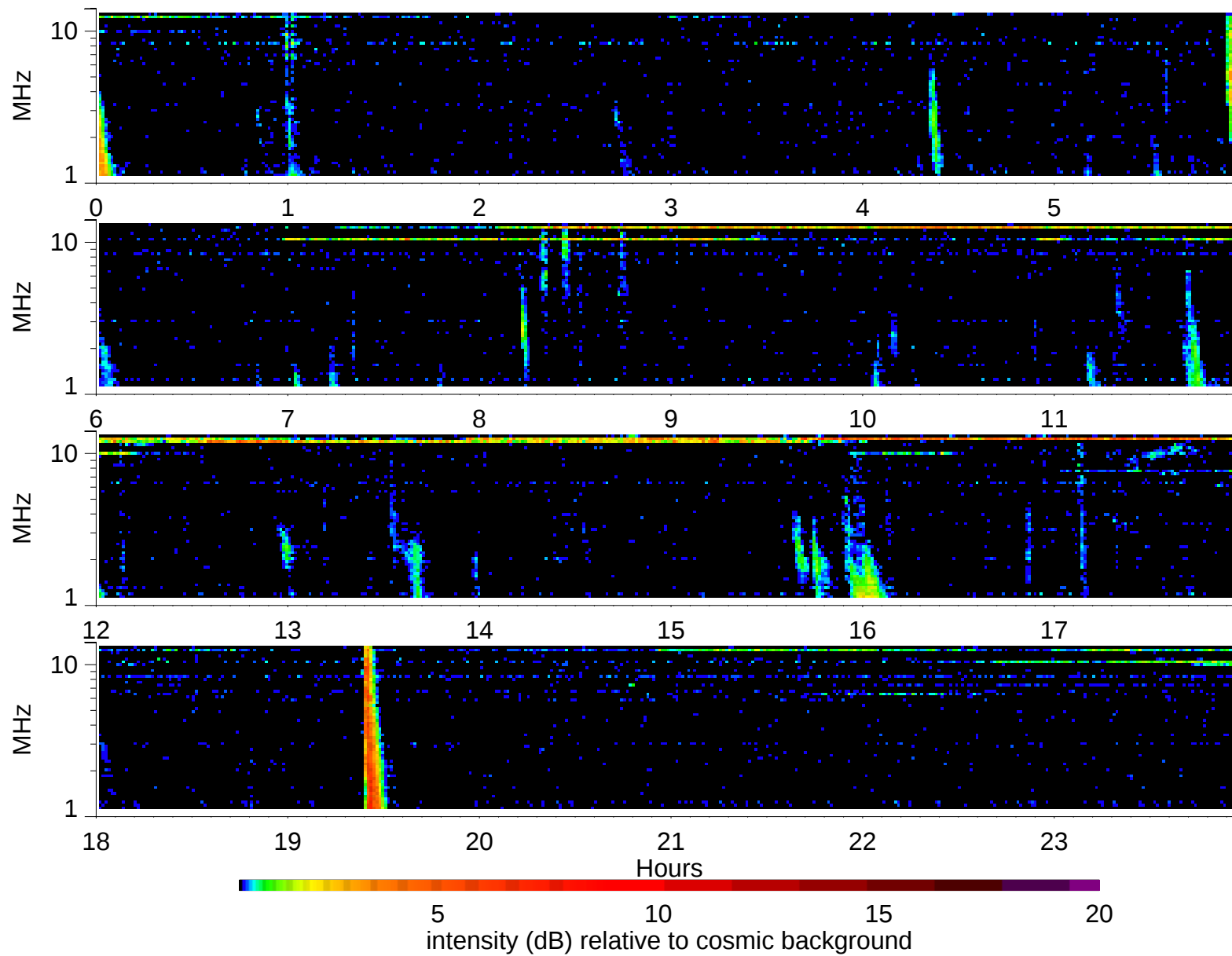
Wind Waves RAD2 receiver: 2002/6/22
