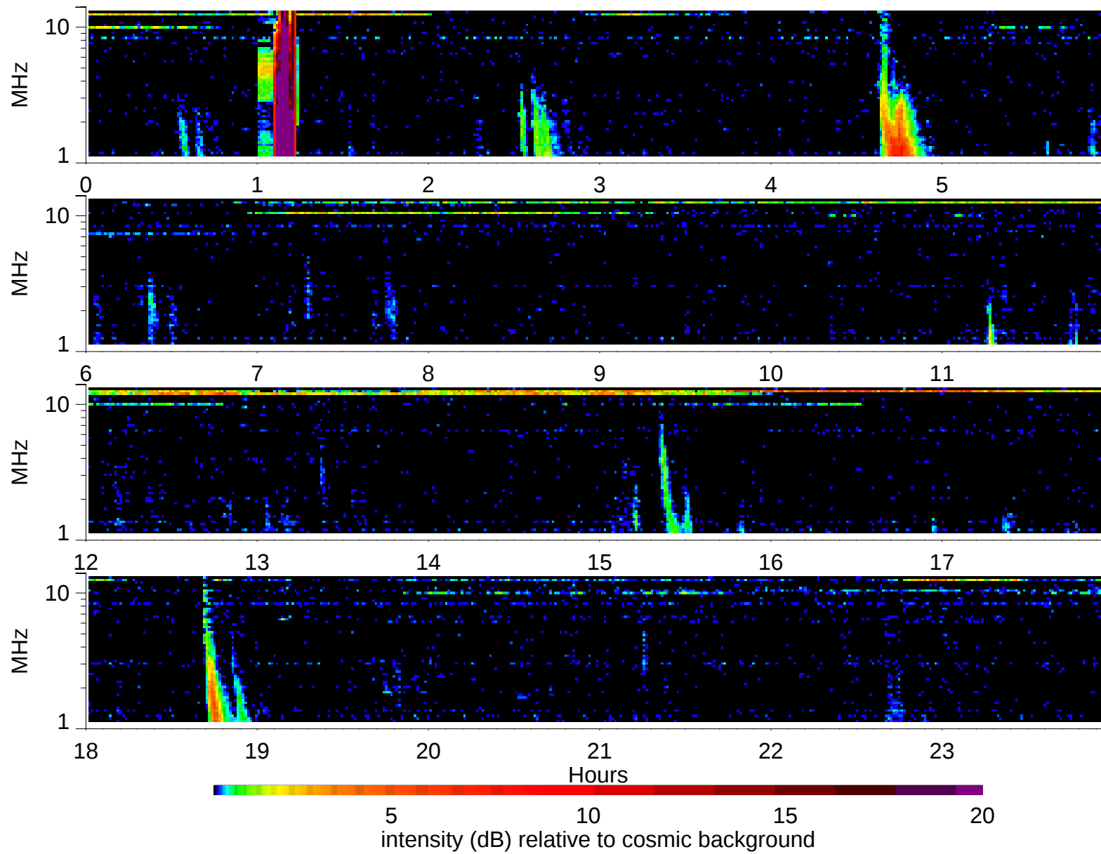
Wind Waves RAD2 receiver: 2002/6/23
