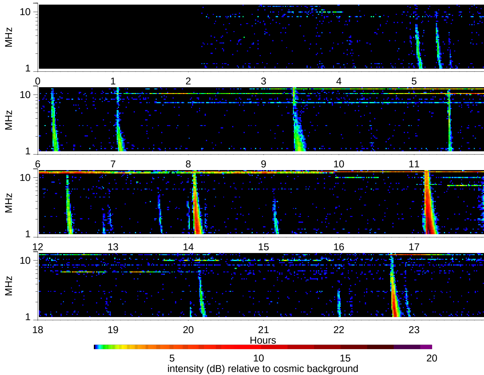
Wind Waves RAD2 receiver: 2002/6/25
