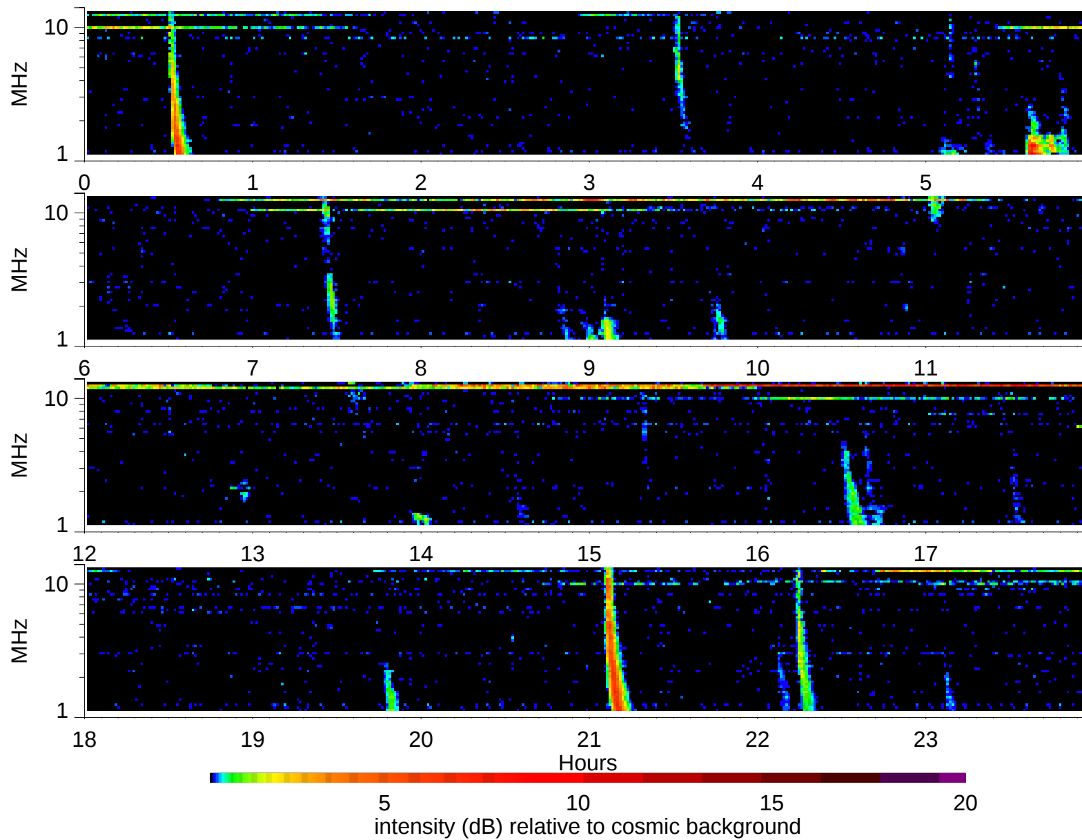
Wind Waves RAD2 receiver: 2002/6/30
