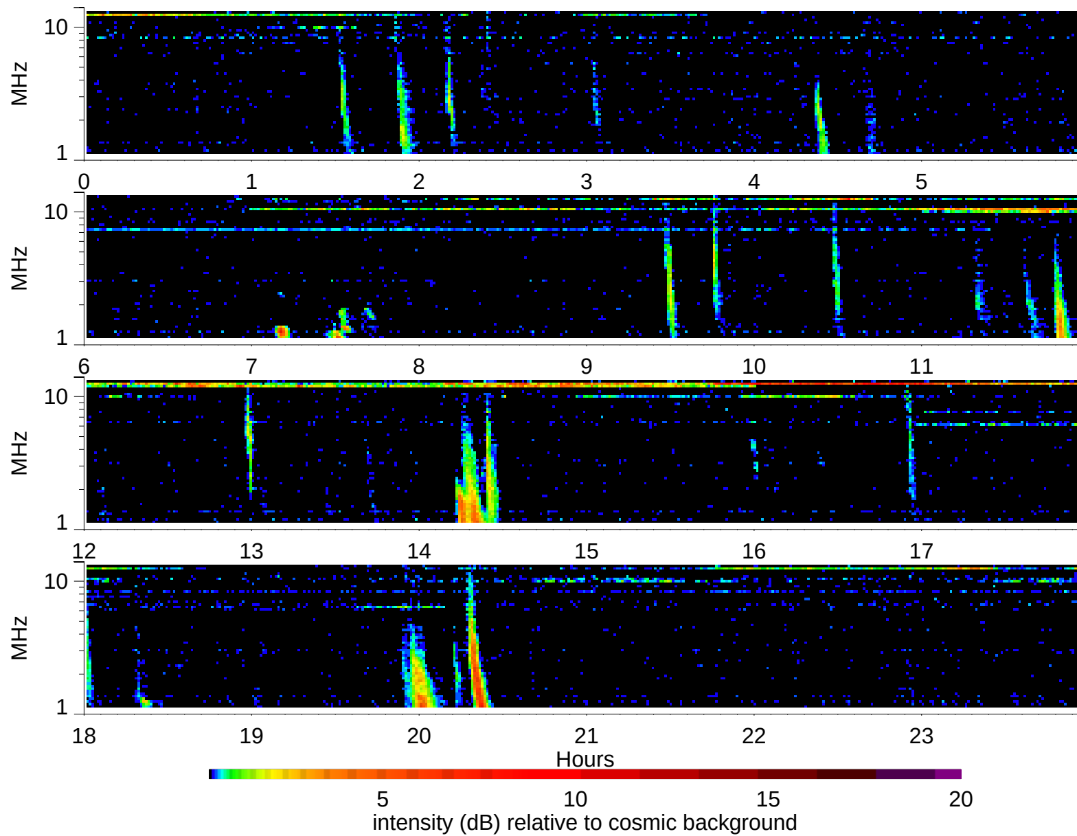
Wind Waves RAD2 receiver: 2002/7/2
