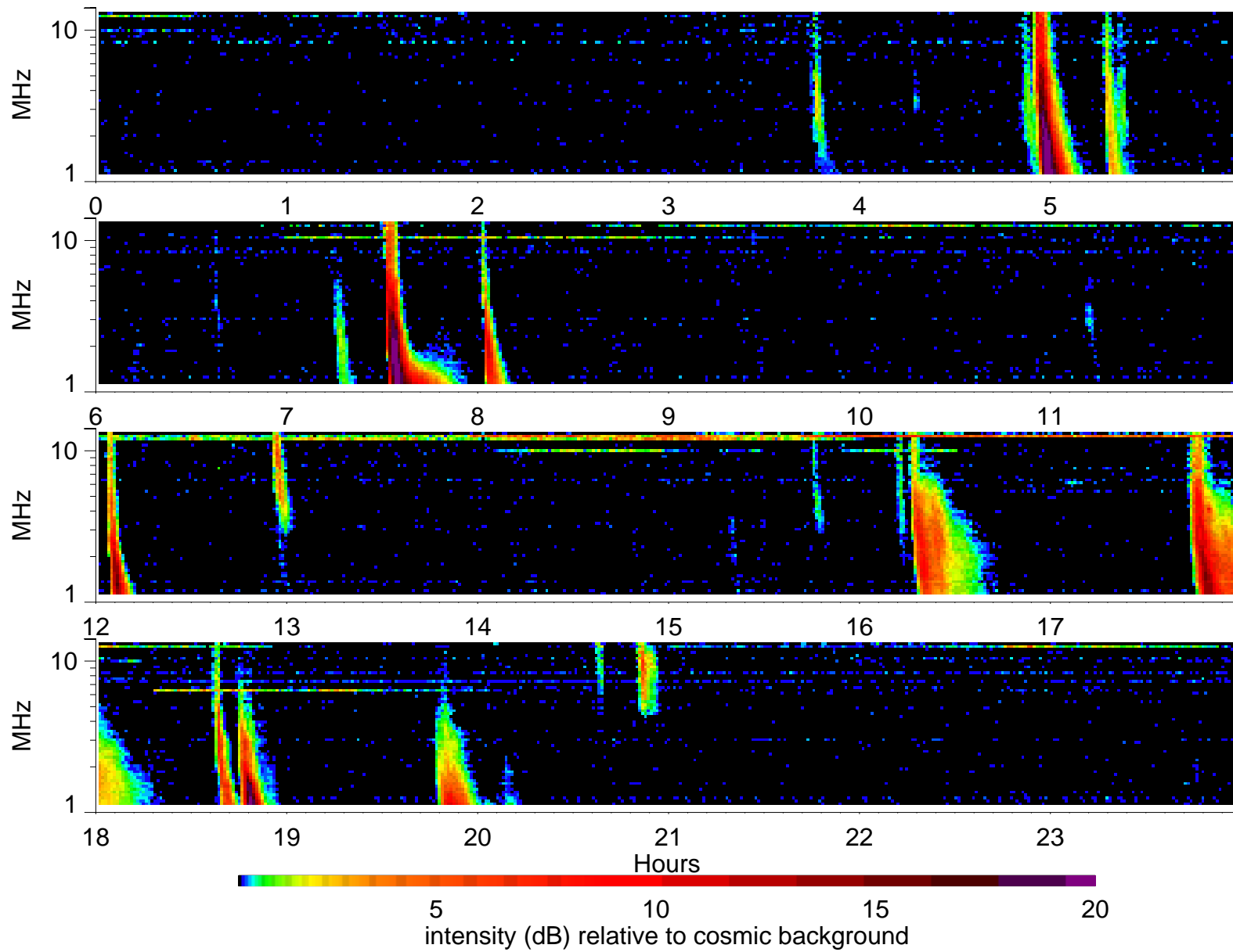
Wind Waves RAD2 receiver: 2002/7/4
