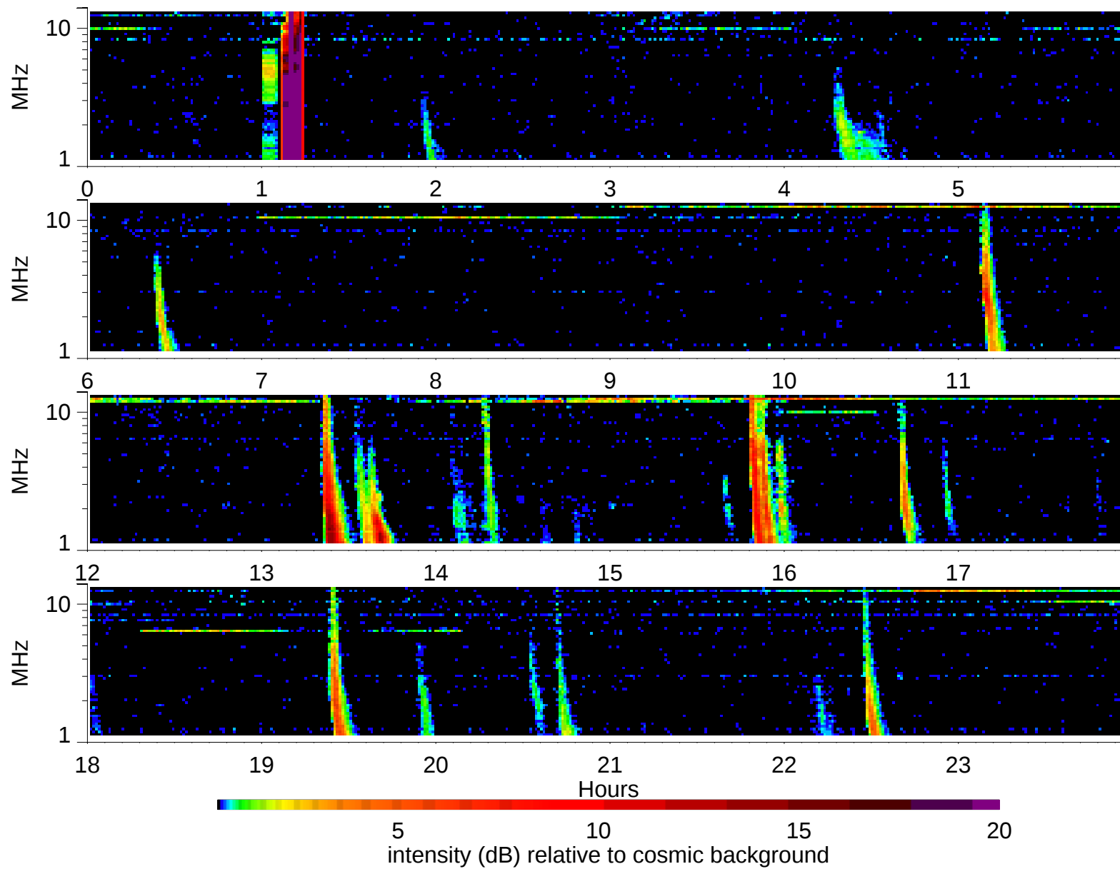
Wind Waves RAD2 receiver: 2002/7/5
