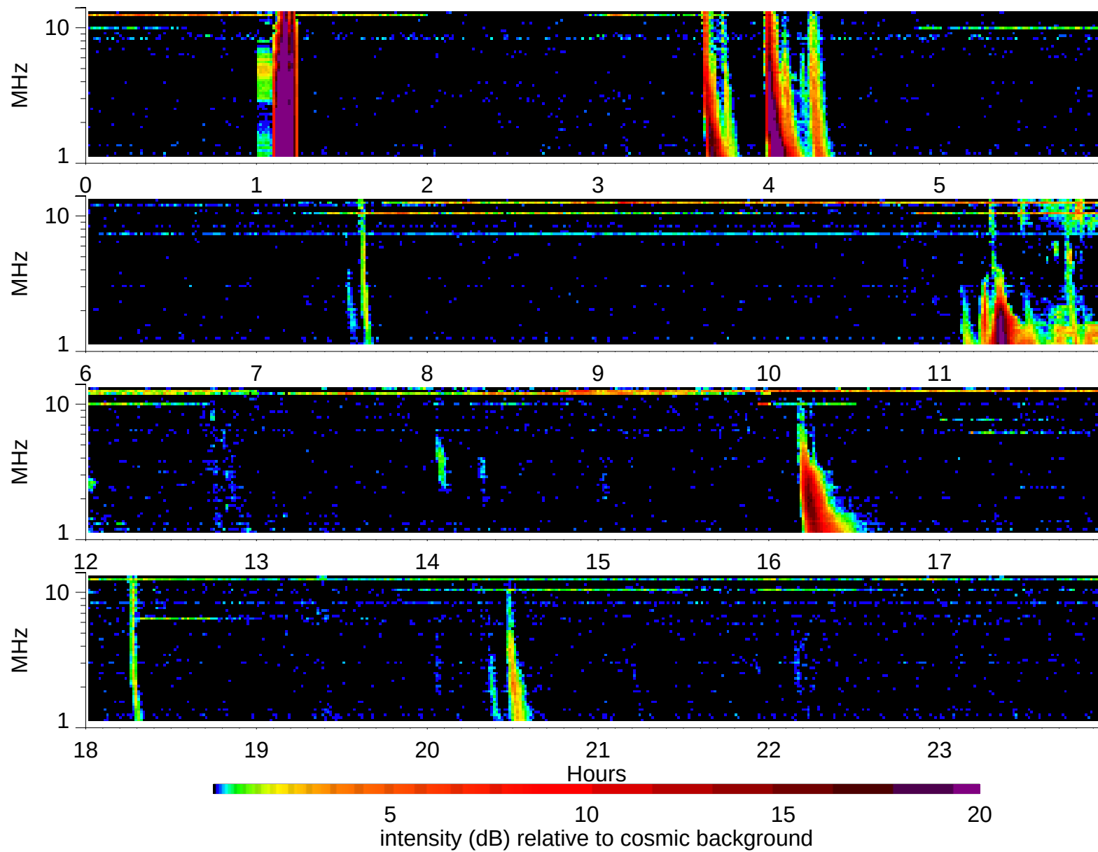
Wind Waves RAD2 receiver: 2002/7/7
