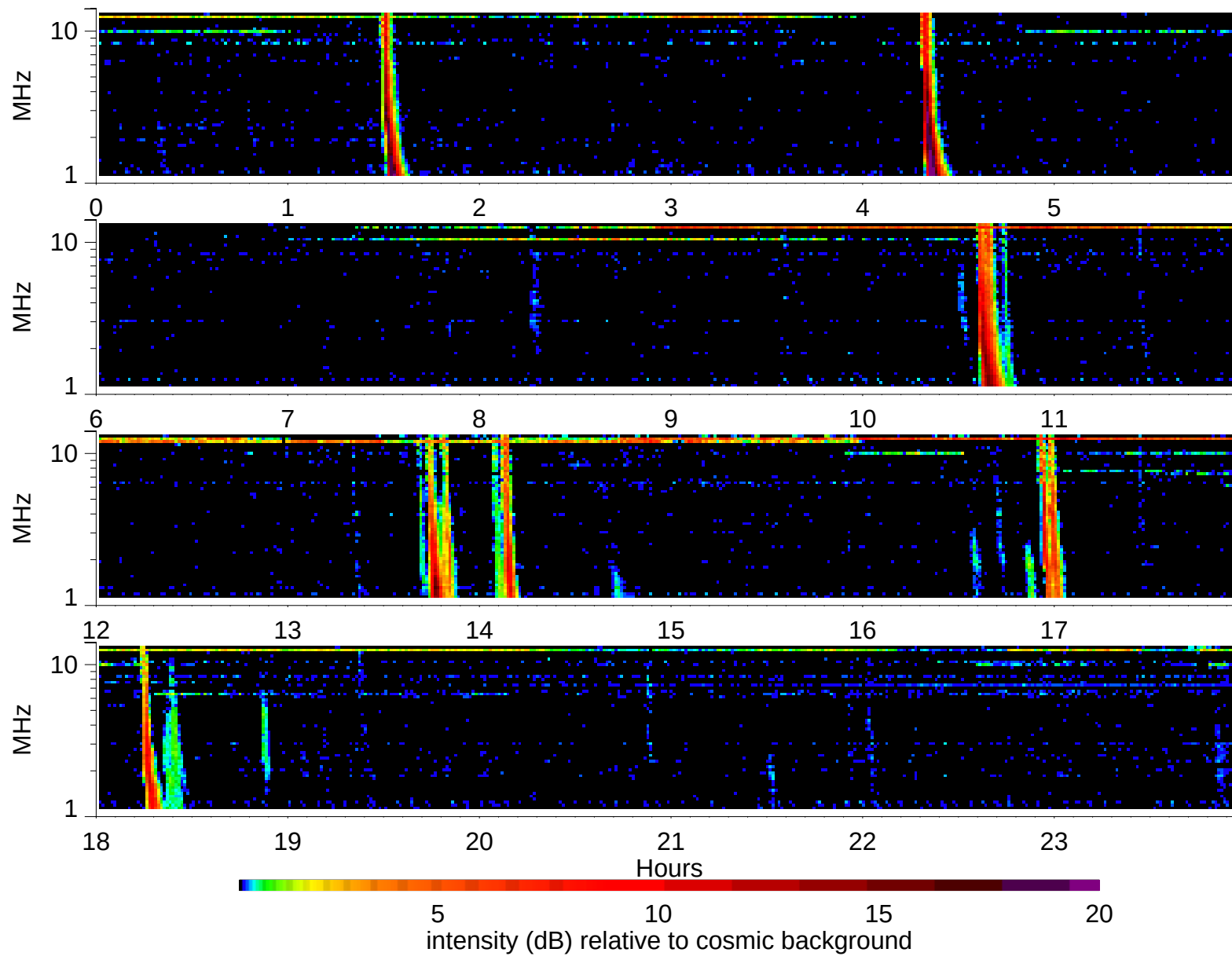
Wind Waves RAD2 receiver: 2002/7/10
