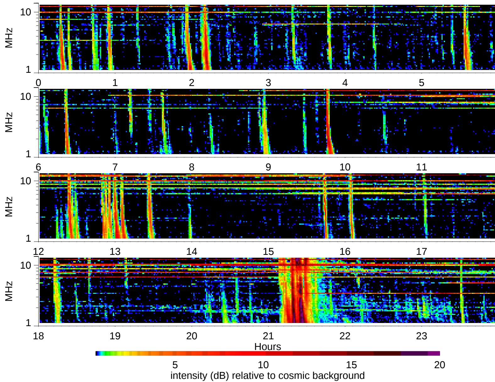
Wind Waves RAD2 receiver: 2002/7/20
