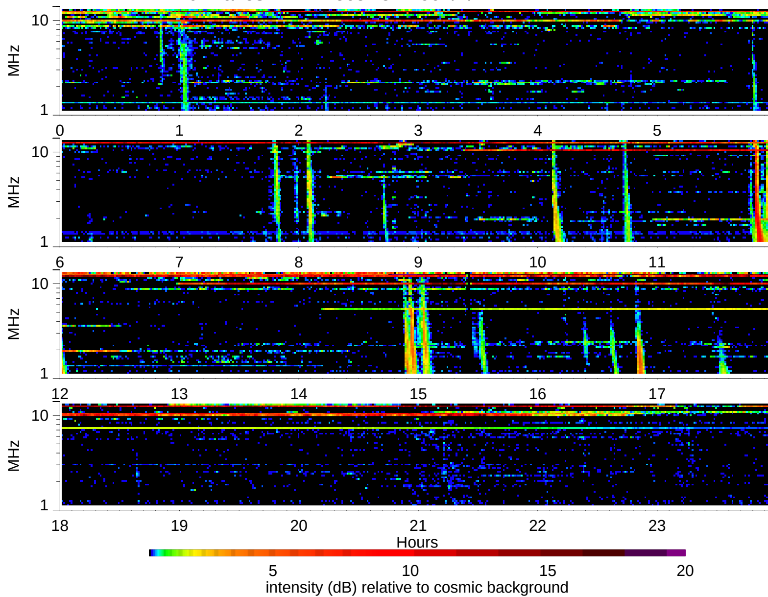
Wind Waves RAD2 receiver: 2002/7/22
