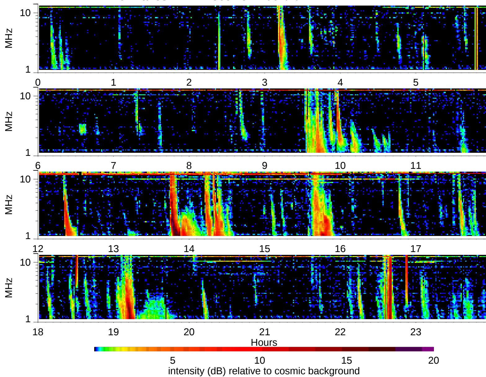
Wind Waves RAD2 receiver: 2002/7/24
