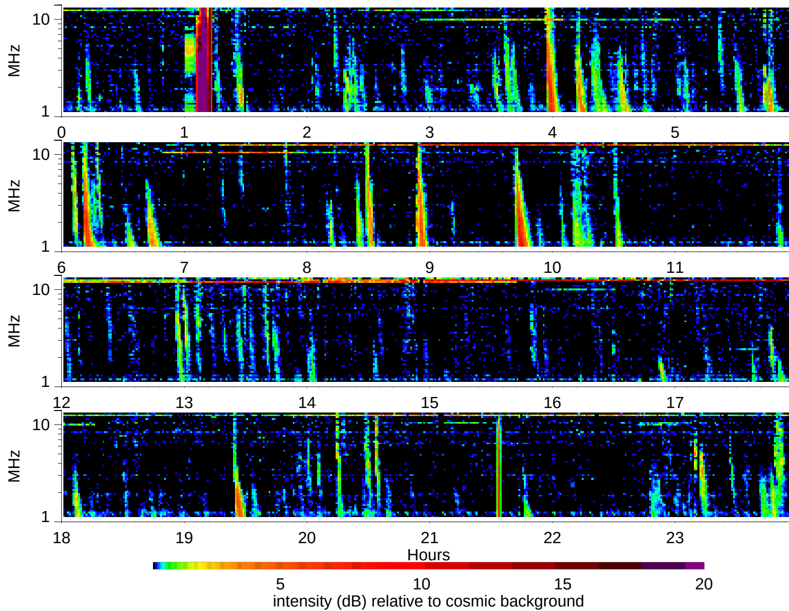
Wind Waves RAD2 receiver: 2002/7/25
