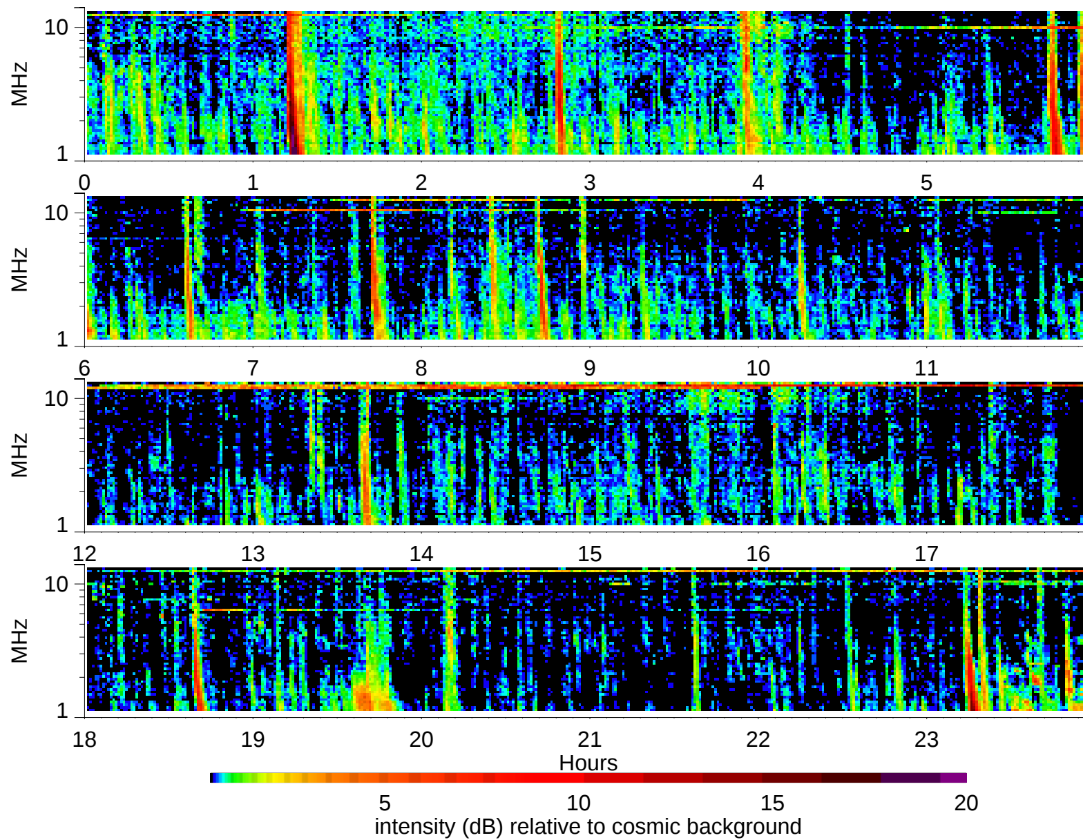
Wind Waves RAD2 receiver: 2002/7/28
