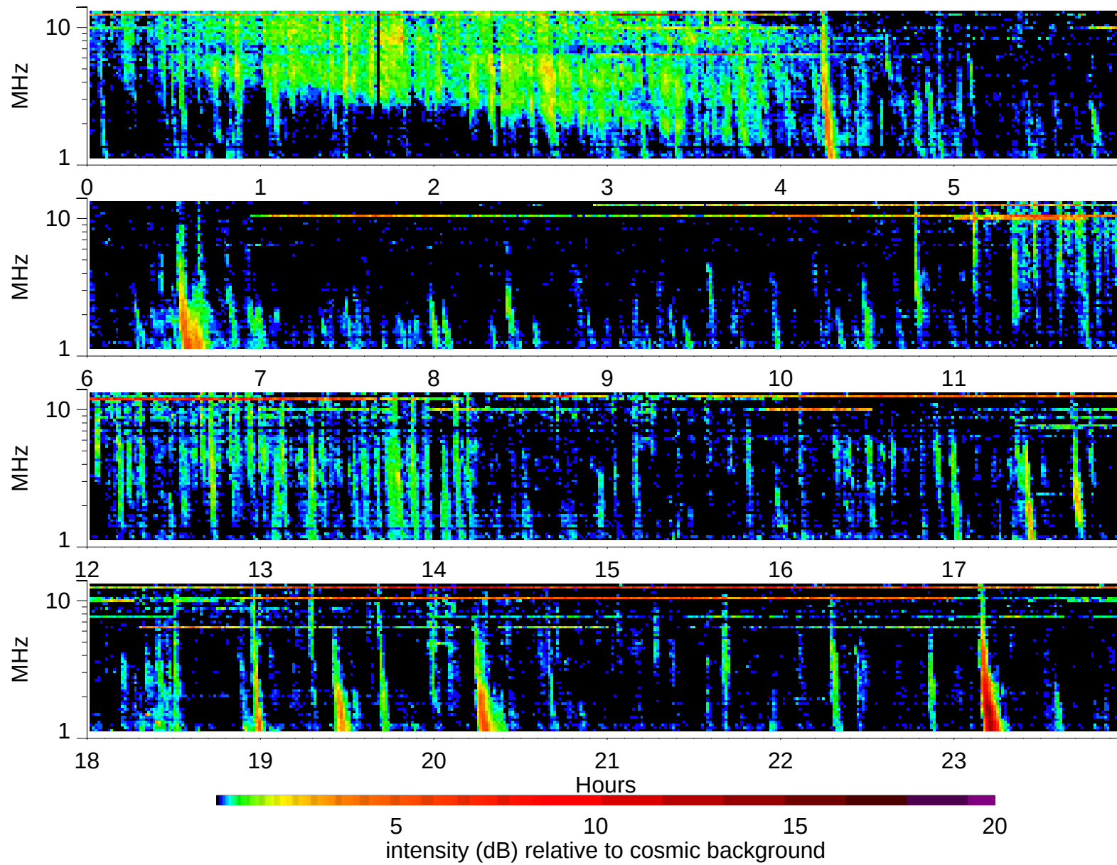
Wind Waves RAD2 receiver: 2002/8/7
