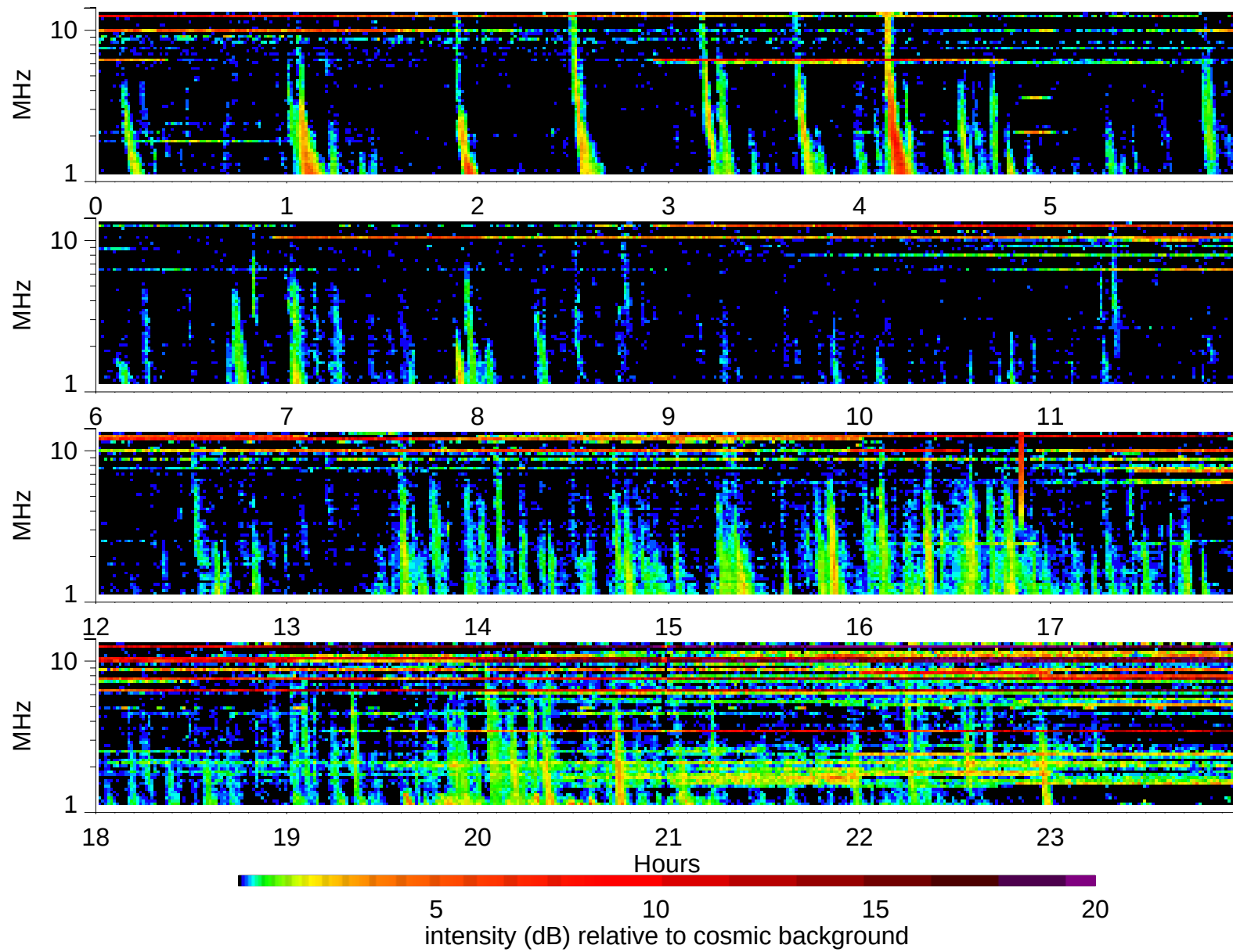
Wind Waves RAD2 receiver: 2002/8/9
