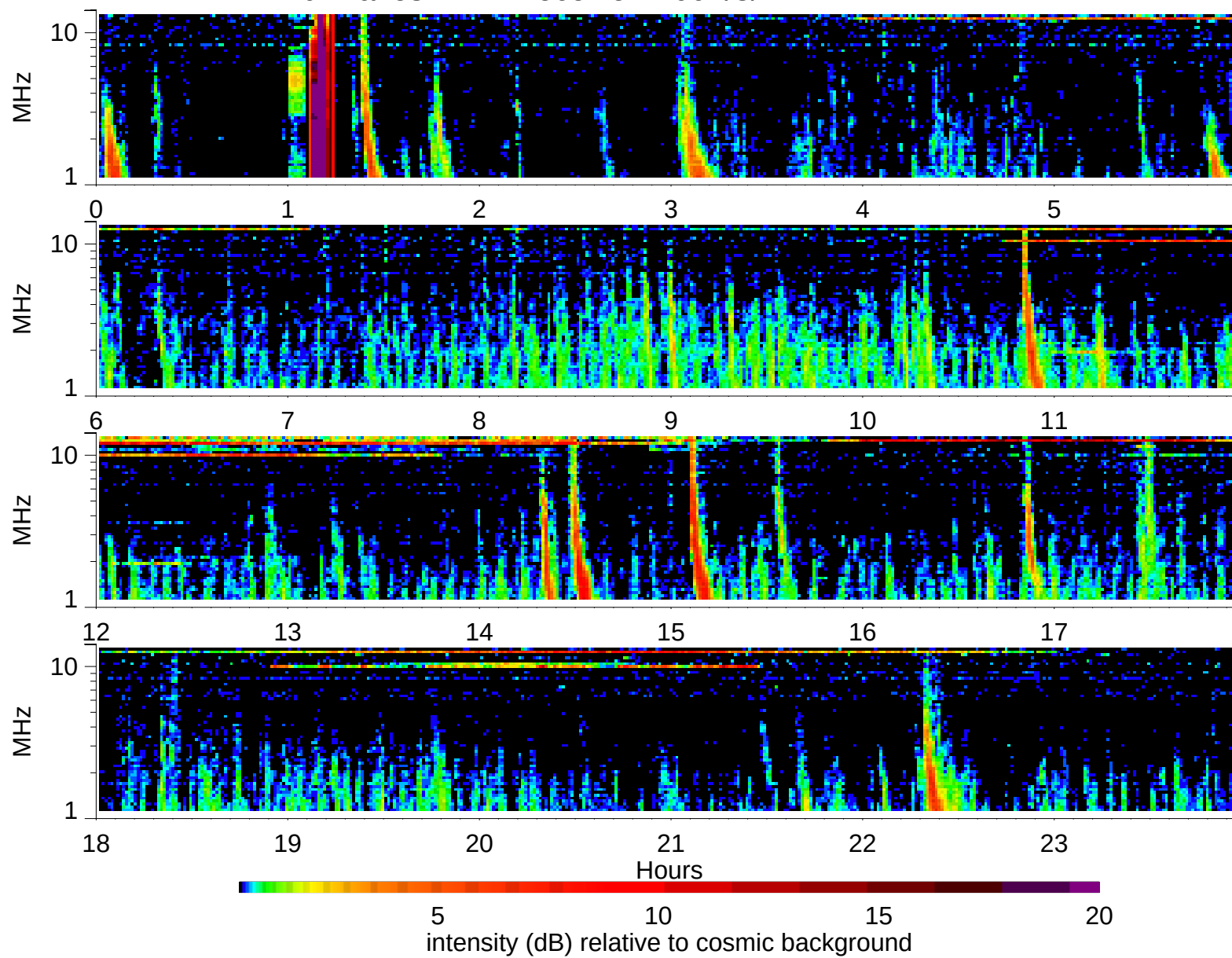
Wind Waves RAD2 receiver: 2002/8/12
