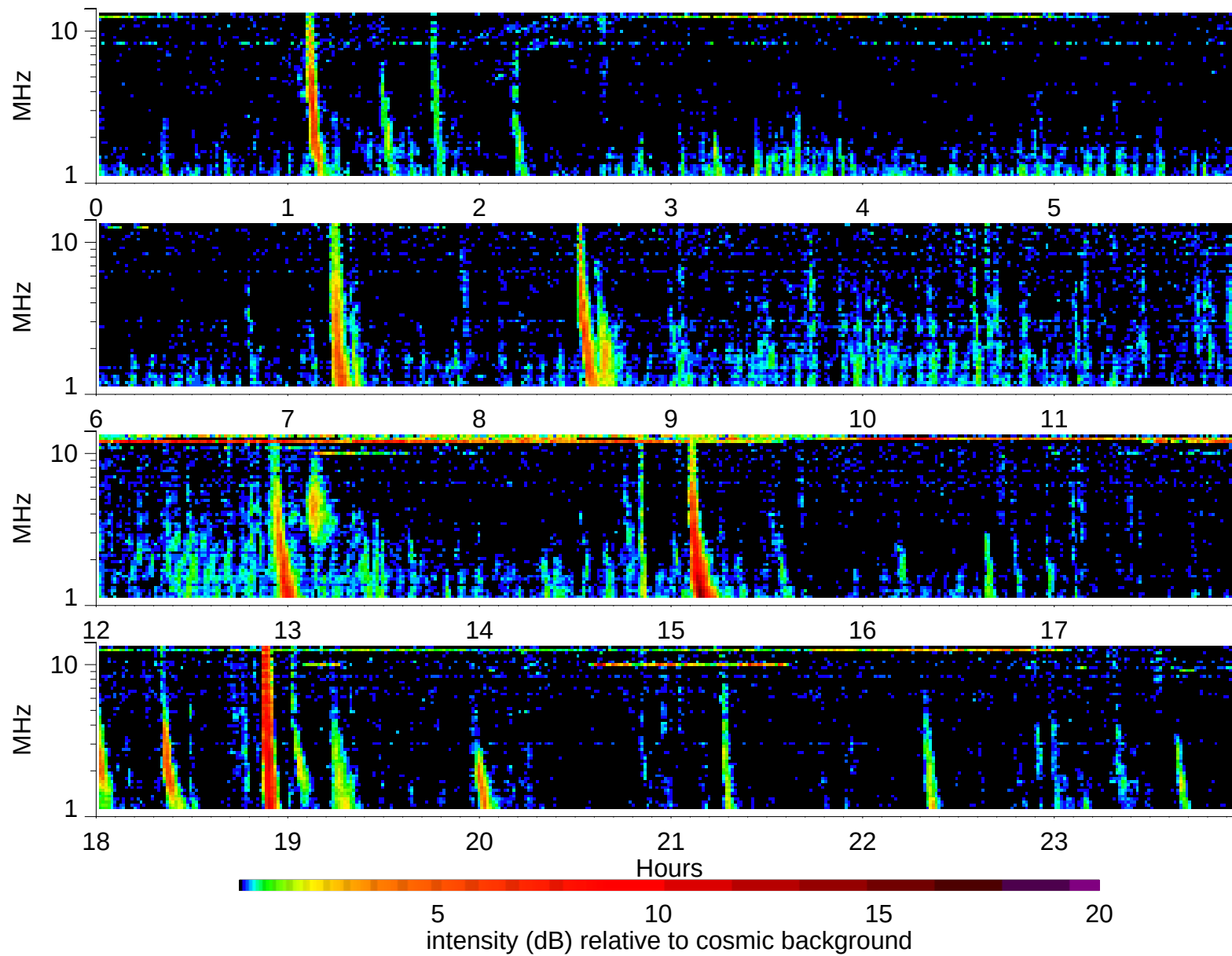
Wind Waves RAD2 receiver: 2002/8/13
