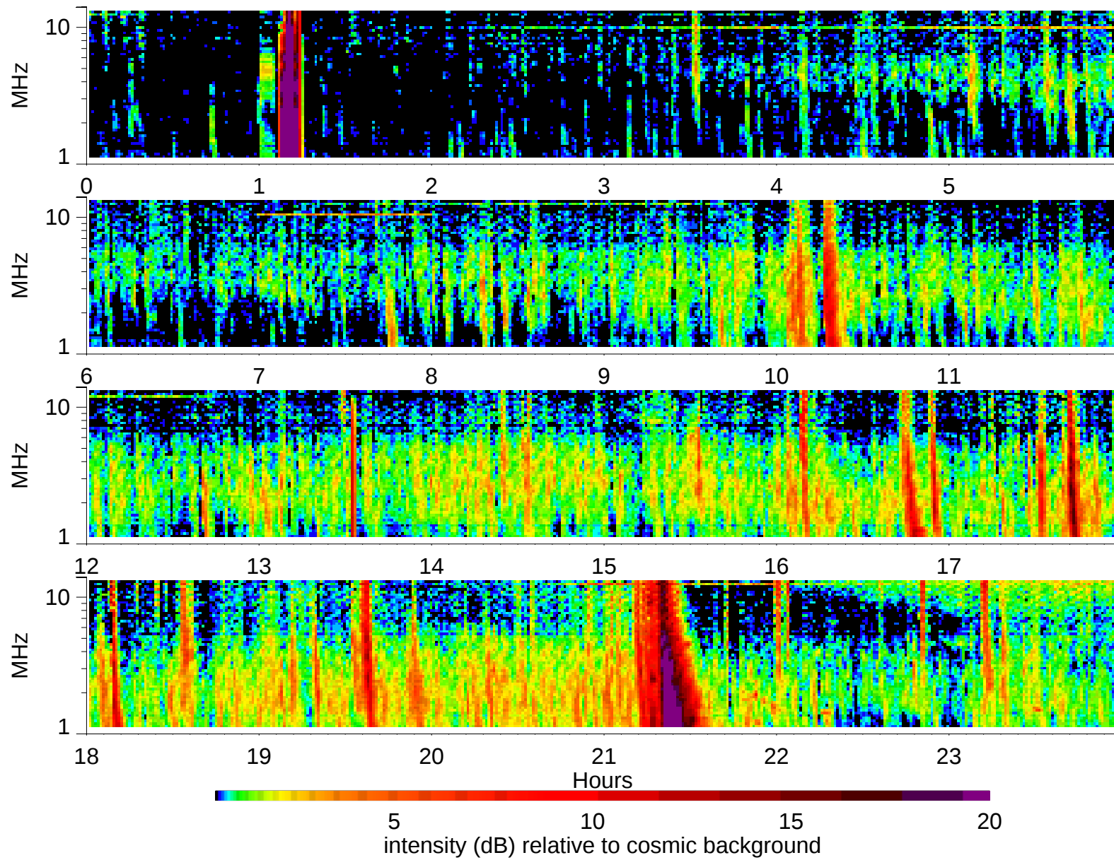
Wind Waves RAD2 receiver: 2002/8/18
