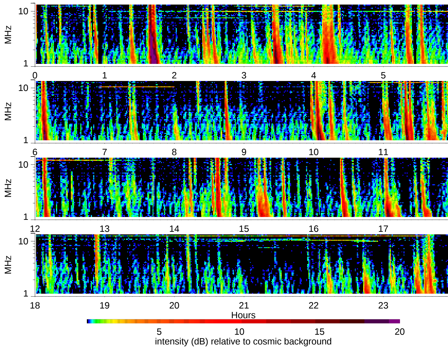
Wind Waves RAD2 receiver: 2002/8/21
