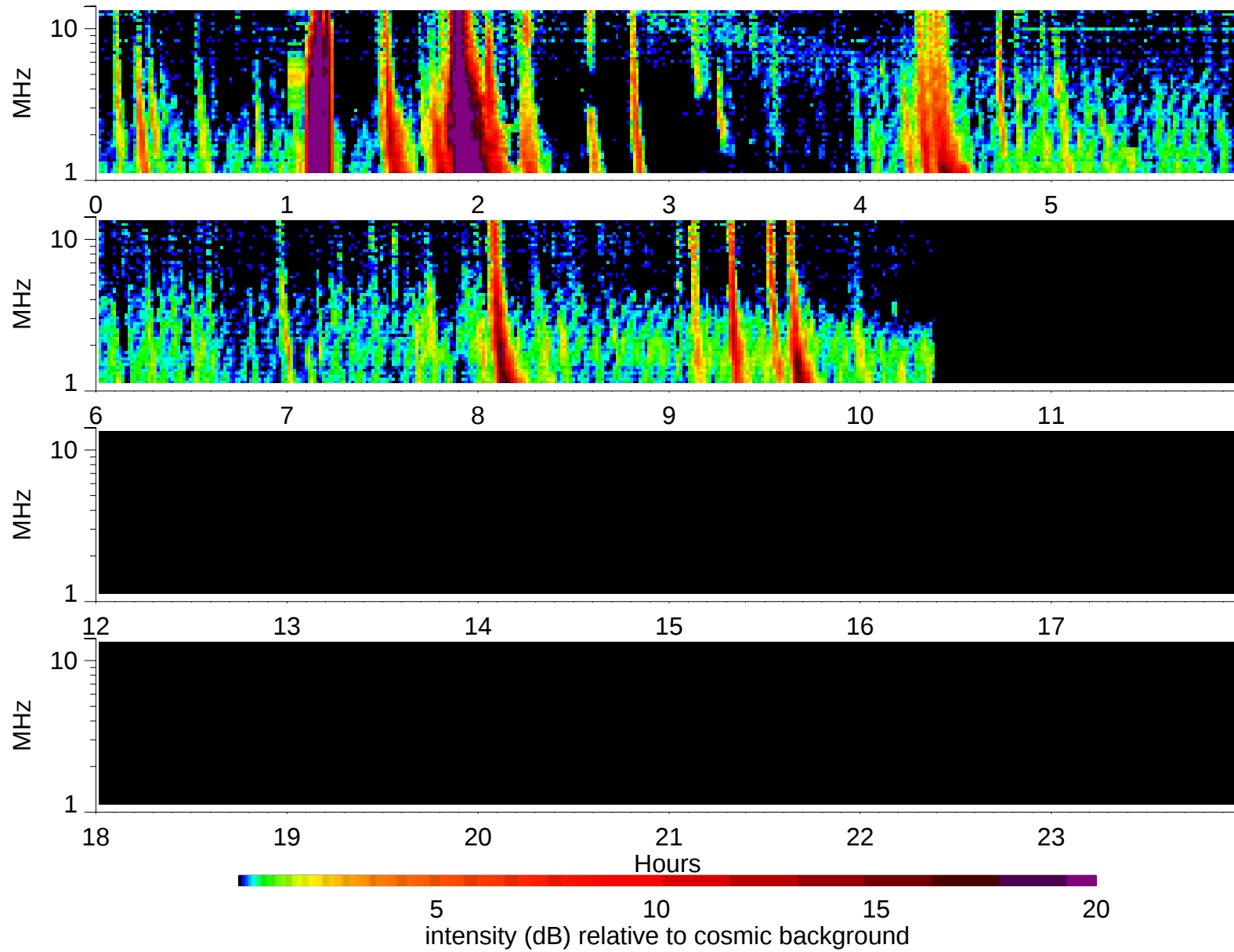
Wind Waves RAD2 receiver: 2002/8/22
