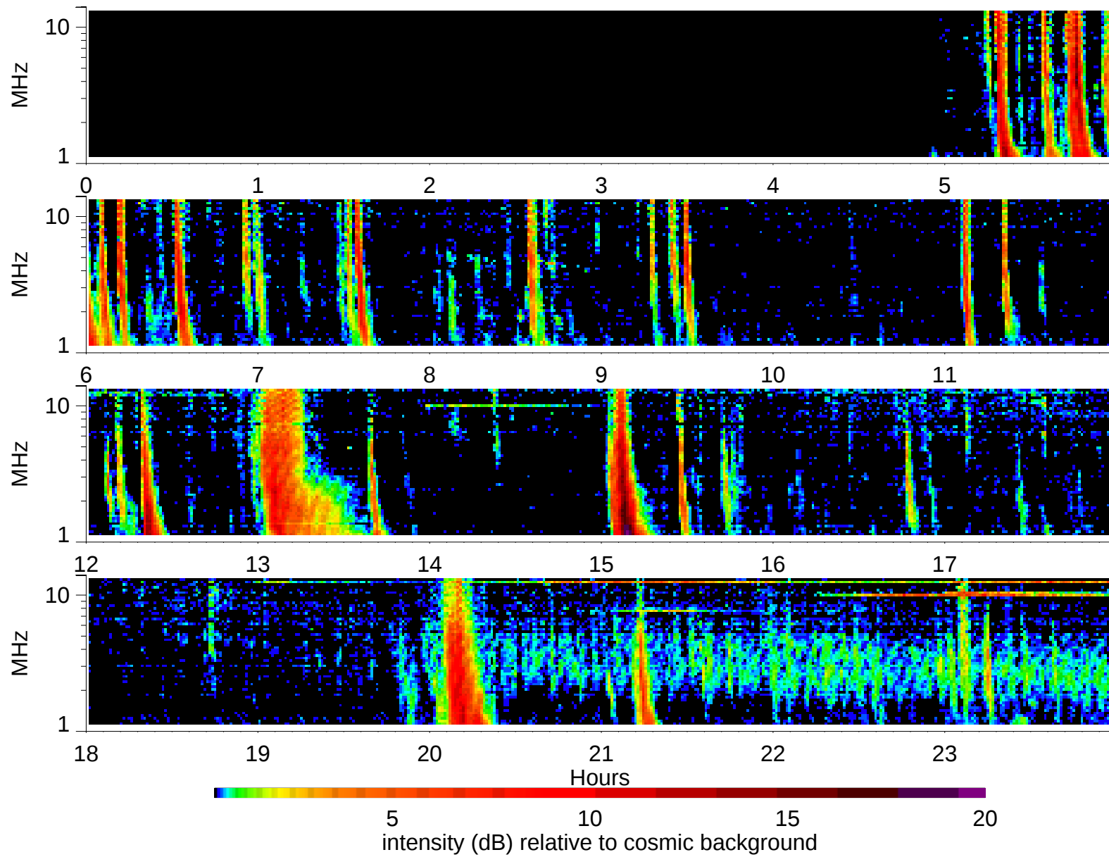
Wind Waves RAD2 receiver: 2002/8/23
