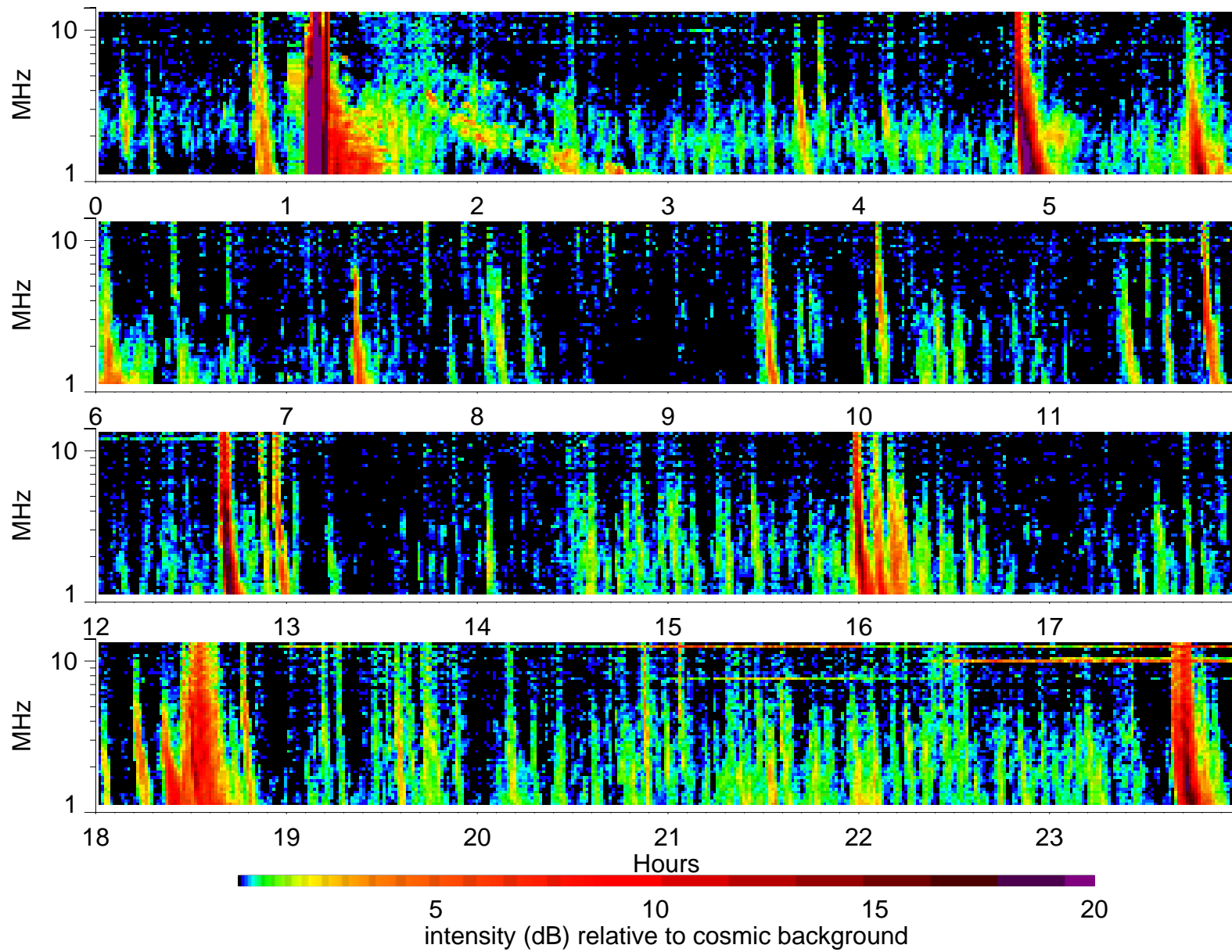
Wind Waves RAD2 receiver: 2002/8/24
