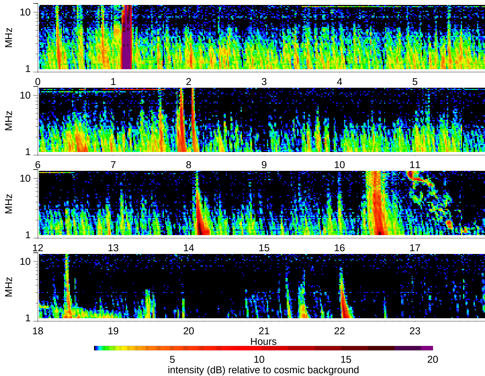
Wind Waves RAD2 receiver: 2002/9/5
