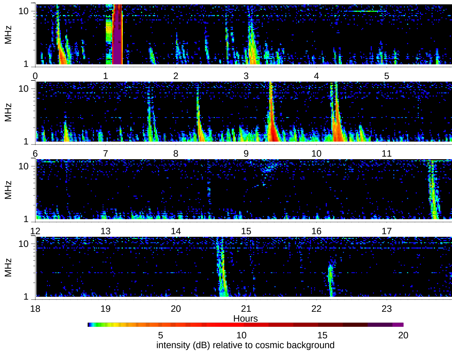
Wind Waves RAD2 receiver: 2002/9/7
