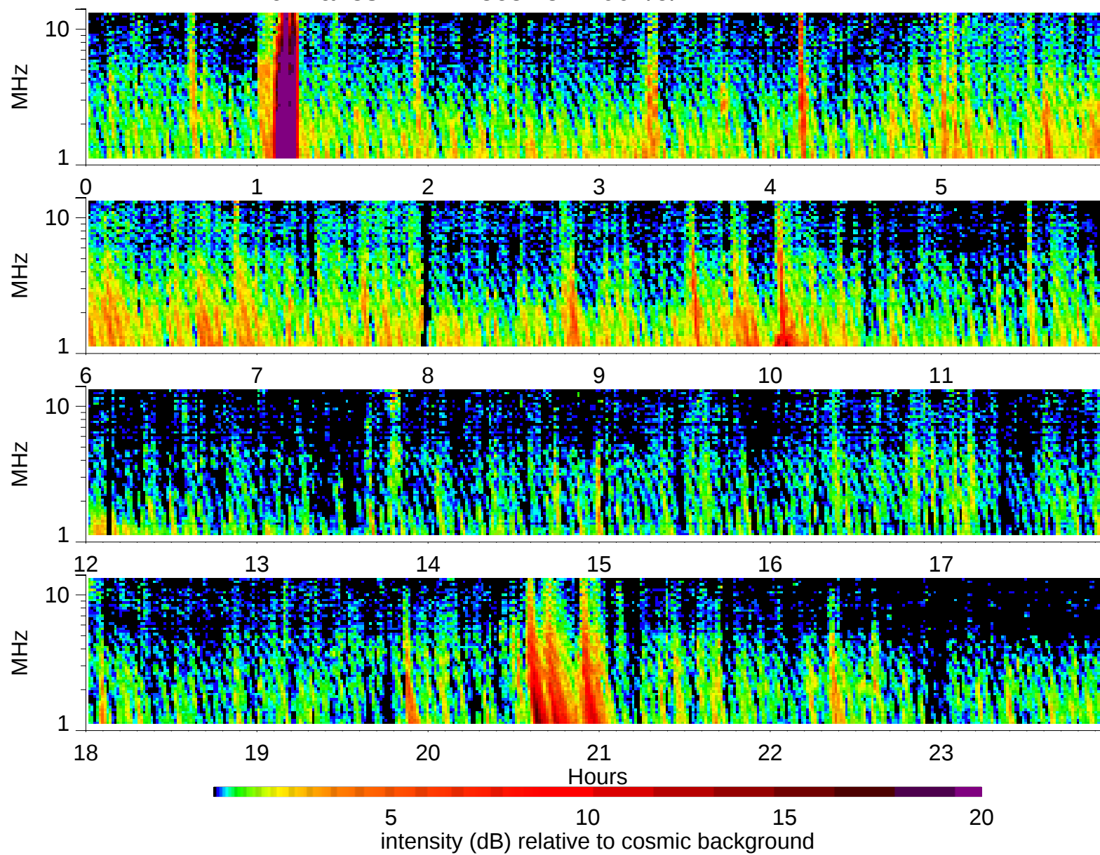
Wind Waves RAD2 receiver: 2002/9/21
