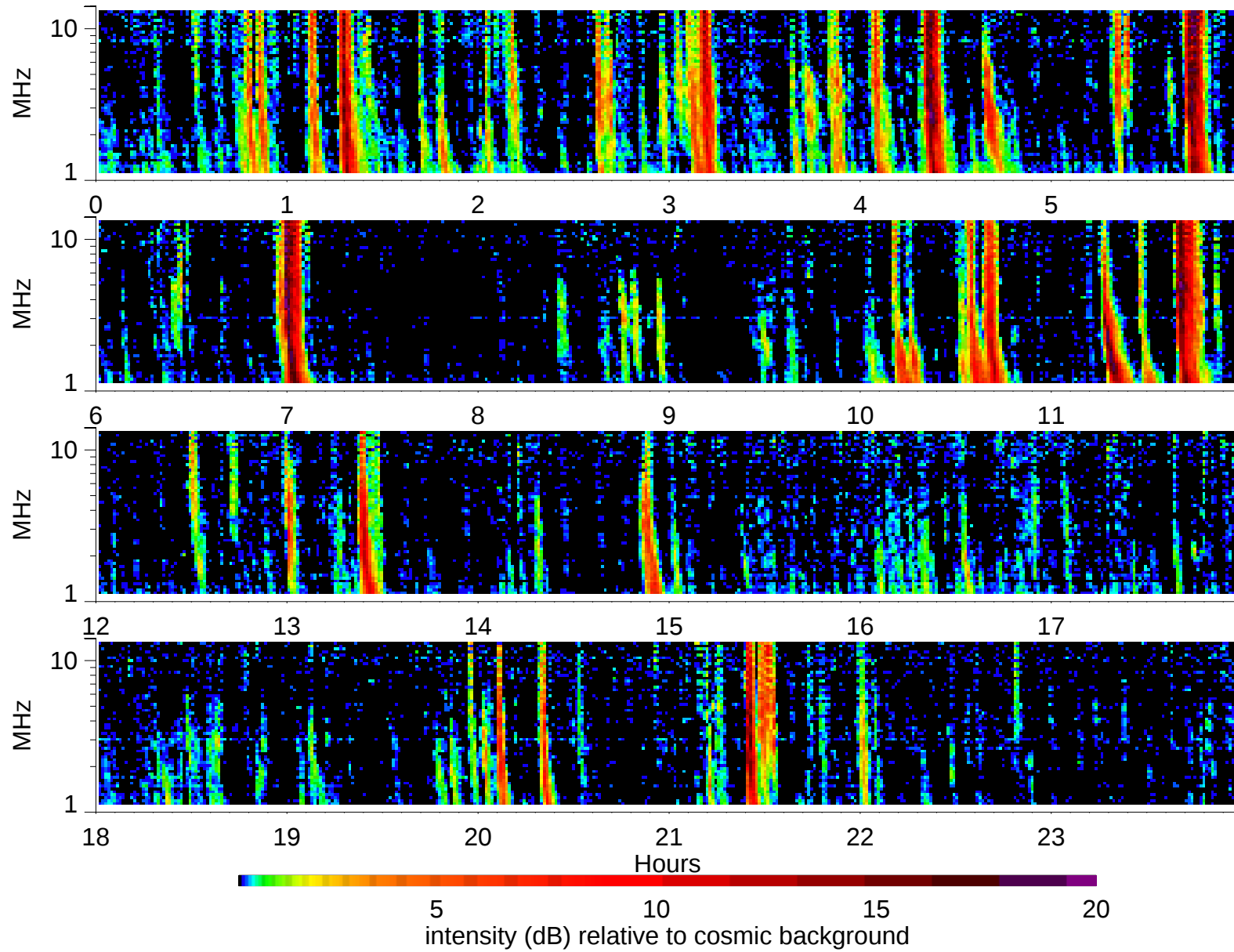
Wind Waves RAD2 receiver: 2002/9/30
