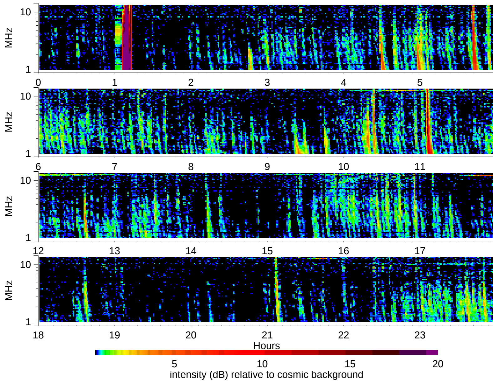
Wind Waves RAD2 receiver: 2002/10/1
