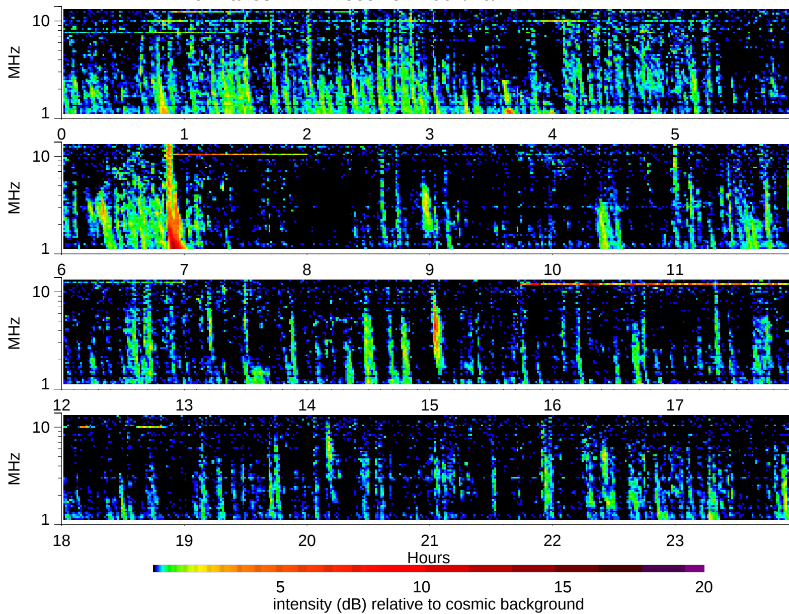
Wind Waves RAD2 receiver: 2002/10/2
