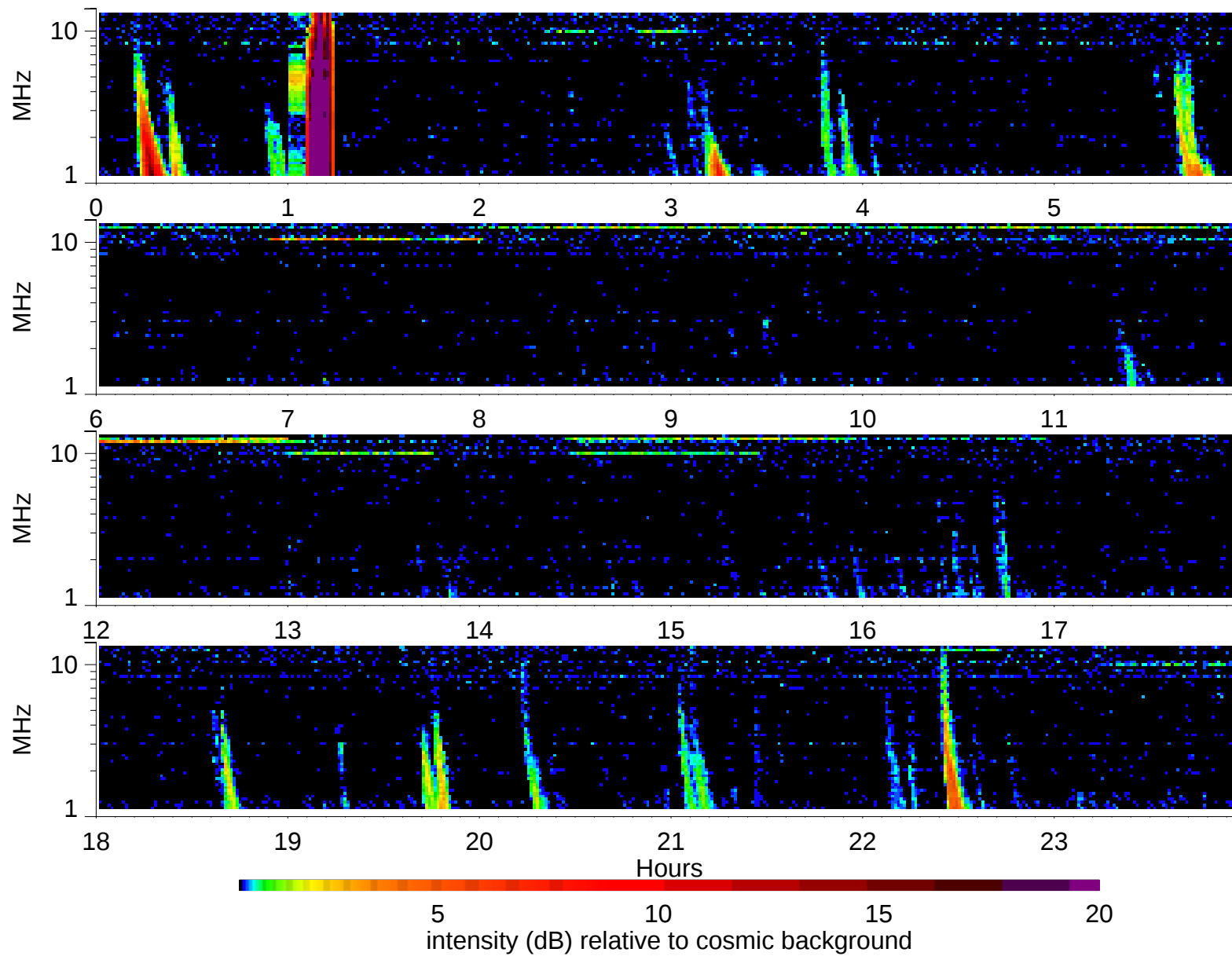
Wind Waves RAD2 receiver: 2002/10/7
