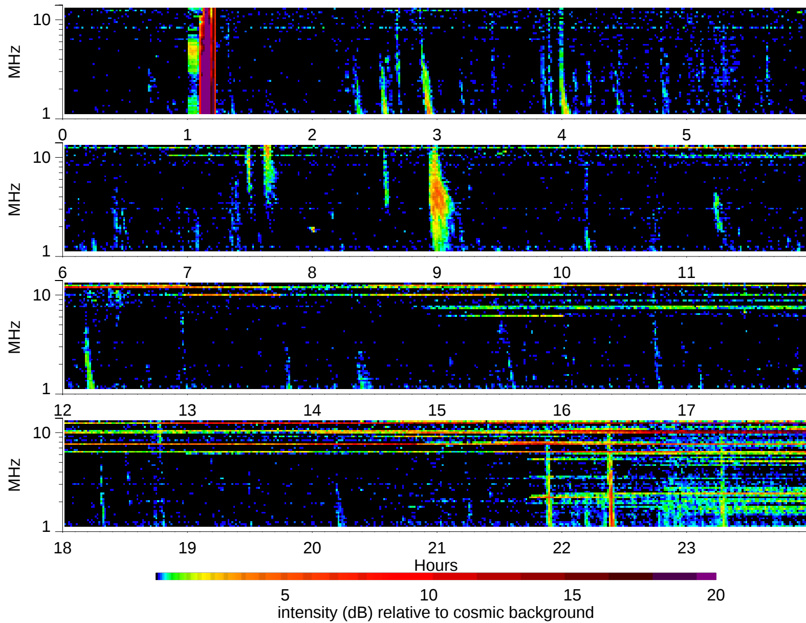
Wind Waves RAD2 receiver: 2002/10/9
