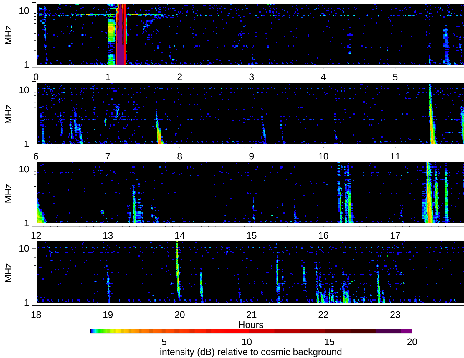
Wind Waves RAD2 receiver: 2002/10/11
