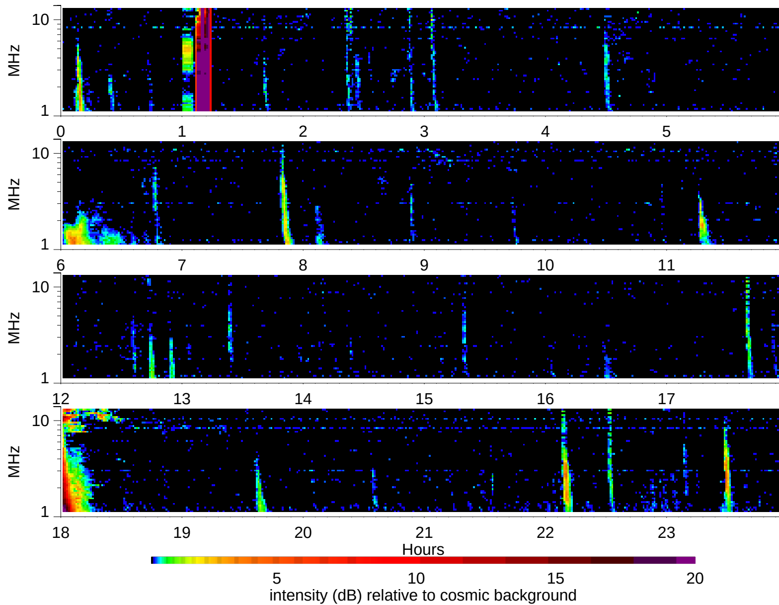
Wind Waves RAD2 receiver: 2002/10/13
